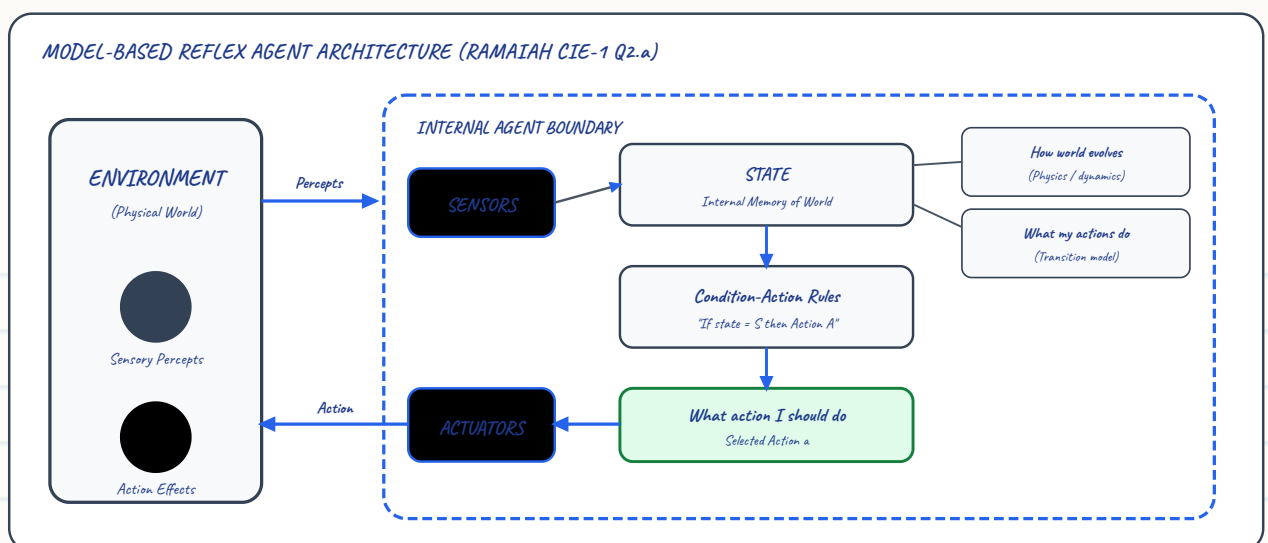
Figure 1.2: Model-Based Reflex Agent Internal Architecture (Ramaiah CIE-1 Q2.a)
