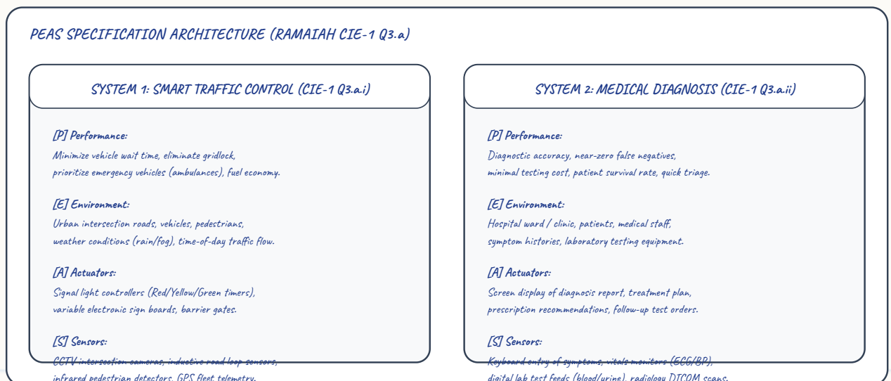
Figure 1.3: PEAS Specification Architecture for Smart Traffic Control & Medical Diagnosis (Ramaiah CIE-1 Q3.a)
