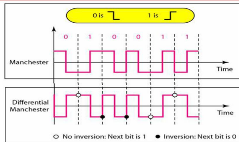
Figure 4.8 Polar biphas: Manchester and differential Manchester schemes
