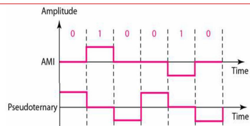
Figure 4.9 Bipolar schemes: AMI and pseudoternary
