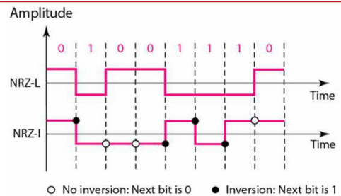
Figure 4.6 Polar NRZ-L and NRZ-I schemes
