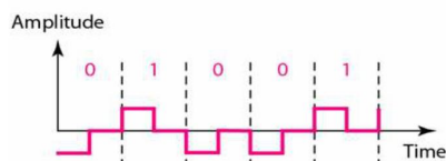
Figure 4.7 Polar RZ scheme
