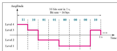
b. A digital signal with four levels
