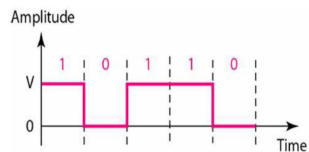
Figure 4.5 Unipolar NRZ scheme
