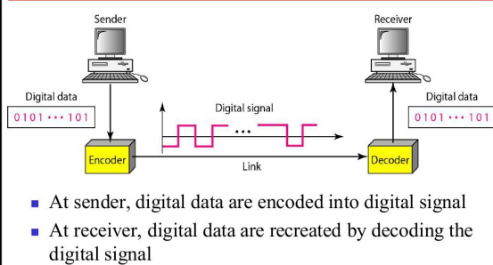
Figure 4.1 Line coding and decoding
