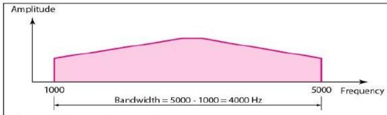
b. Bandwidth of a nonperiodic signal
