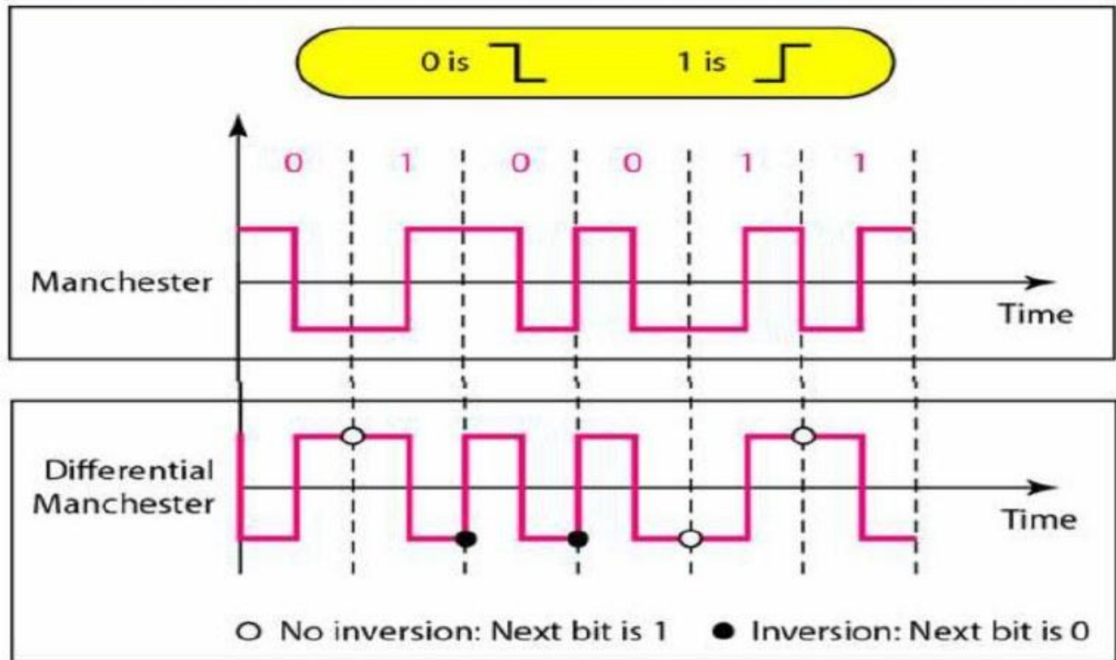
Figure 4.8 Polar biphase: Manchester and differential Manchester schemes
