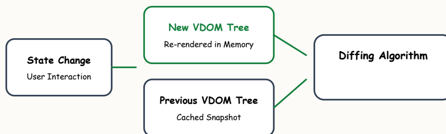
Figure 1.1: The Virtual DOM Diffing and Reconciliation Process
