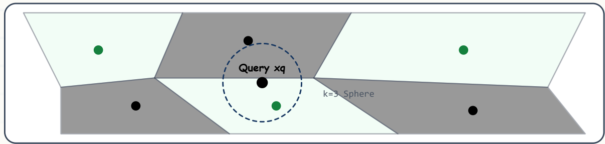
Figure 3.1: Voronoi tessellation: Convex polygonal cells determine nearest-neighbor decision boundaries.
