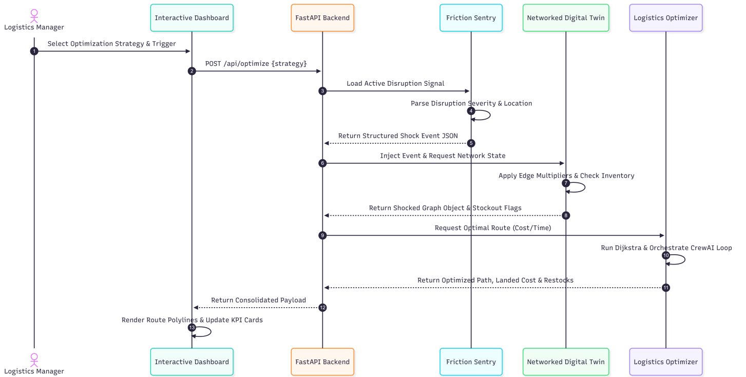
Figure 5.2: Detailed Module Interaction and Data Flow
