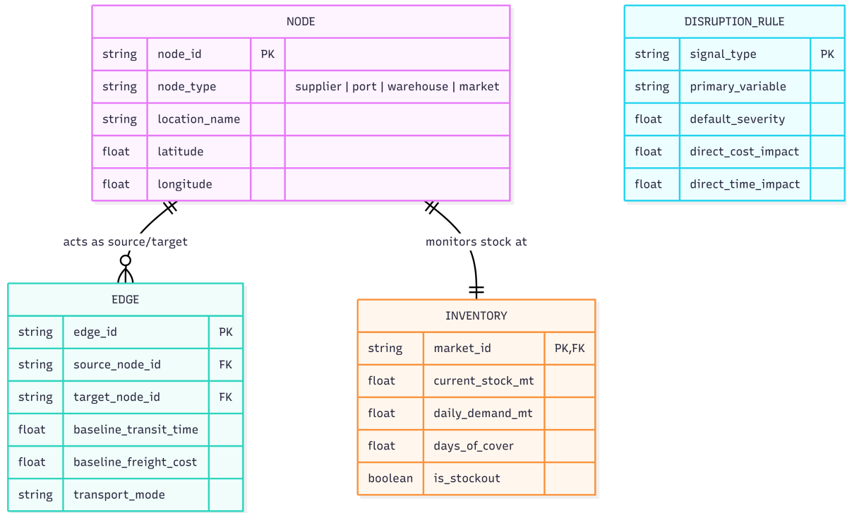
Figure 5.3: Entity-Relationship Diagram for Logistics Digital Twin
