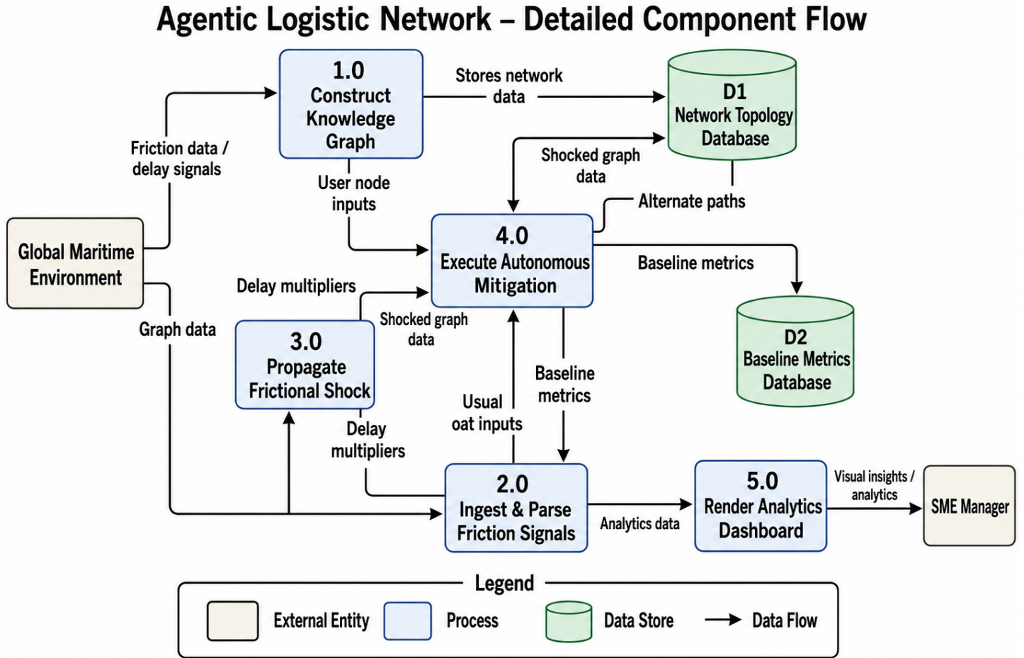
Figure 4.3: Data Flow Diagram Level 1
