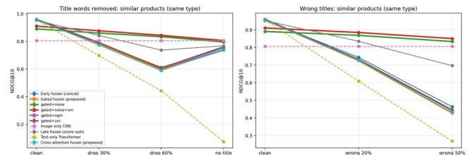
Fig. 4. Similar-product NDCG@10 when title words are removed (left) or titles are wrong (right).
