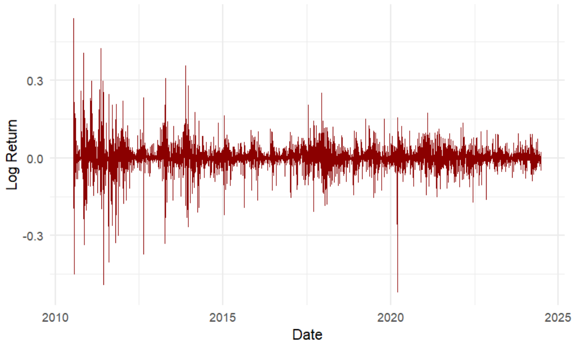
Diagram 3: Bitcoin Daily Log Returns
