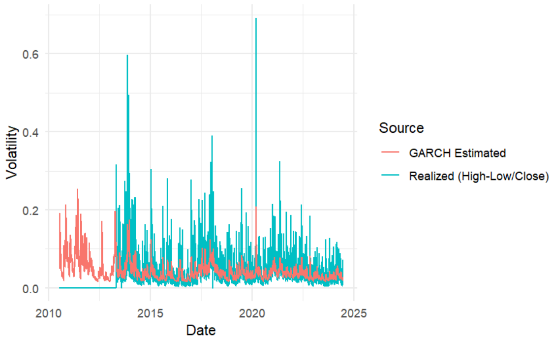
GARCH Estimated Volatility vs Realized Volatility
