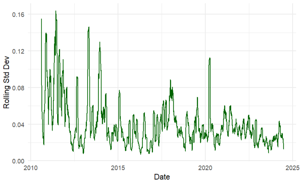
Diagram 5: 30-Day Rolling Volatility of Returns
