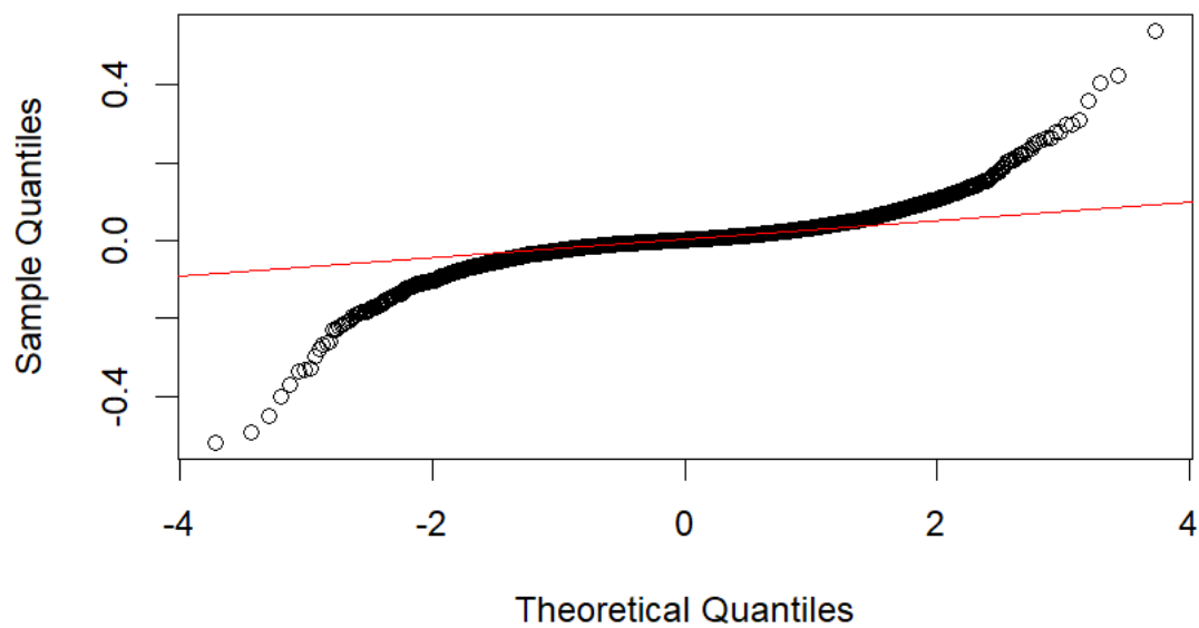
Diagram 6: QQ-Plot of Log Returns
