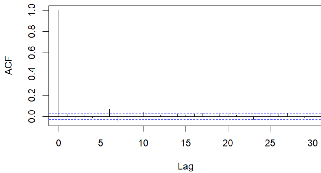
ACF of Log Returns
