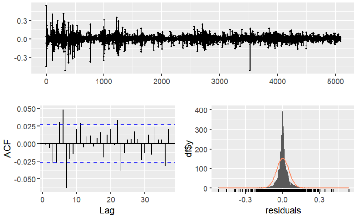
Residuals from ARIMA(2,0,3) with zero mean
