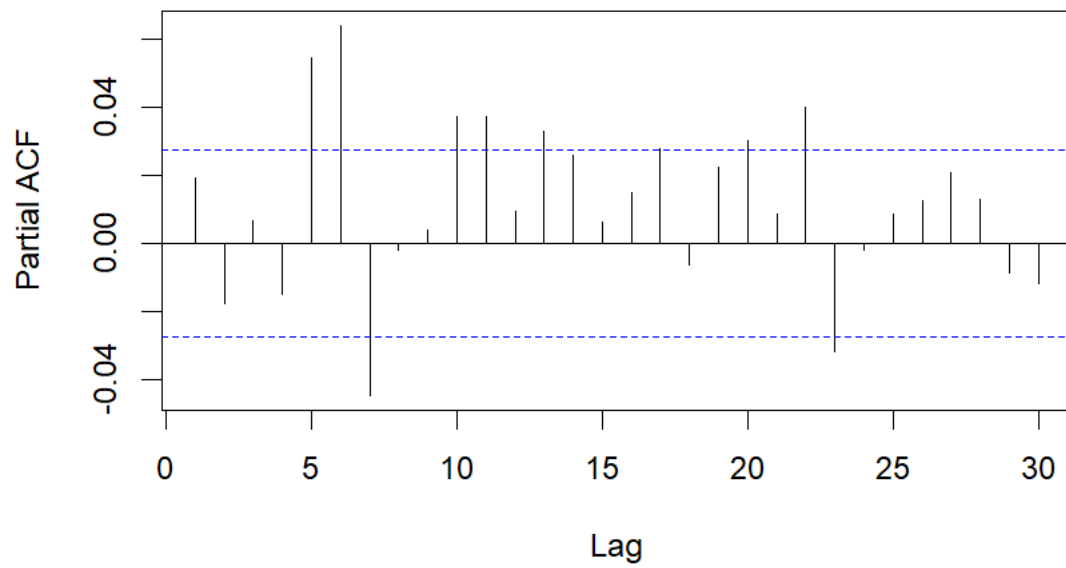
PACF of Log Returns
