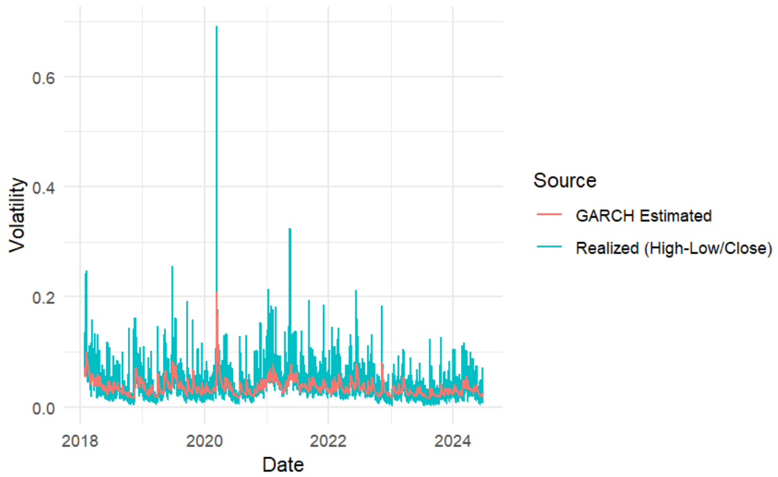
GARCH vs Realized Volatility (Reliable Period Only)
