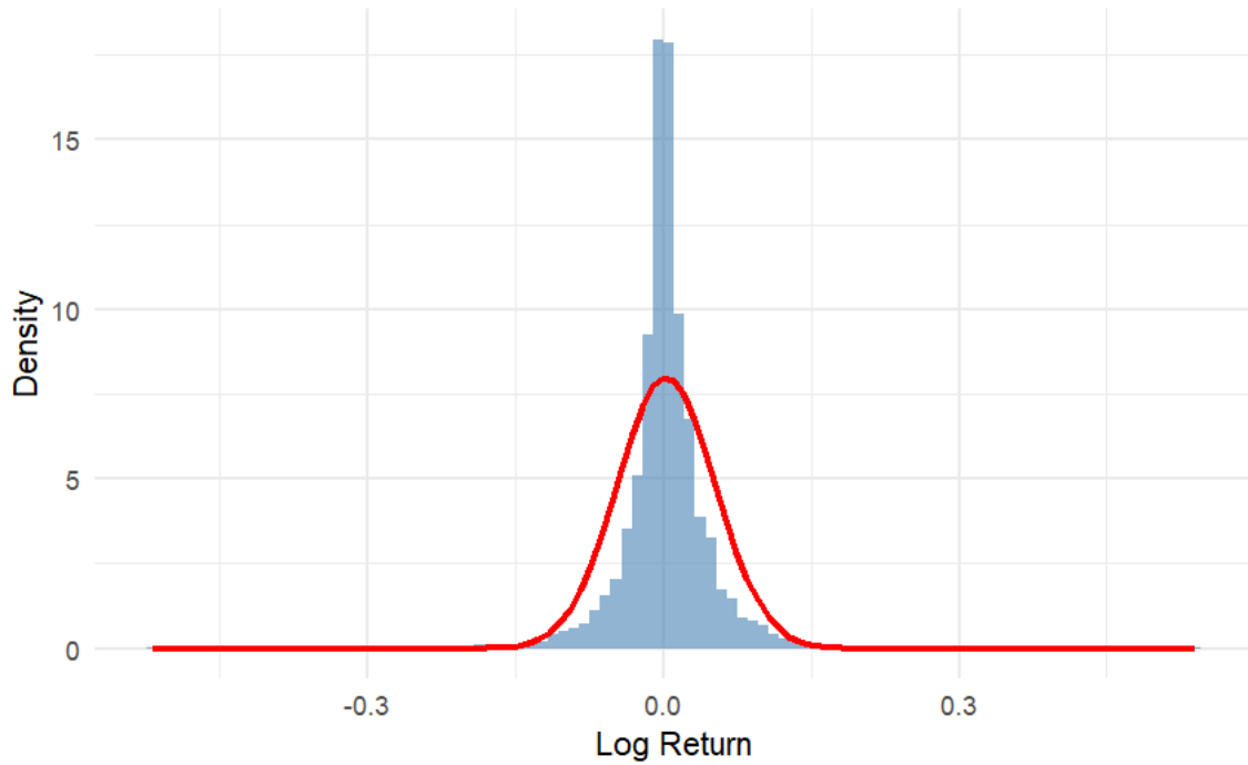
Diagram 4: Distribution of Log Returns vs Normal
