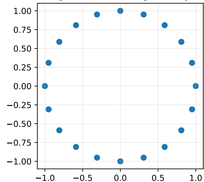
Fig 1C: Metabolite geometry
