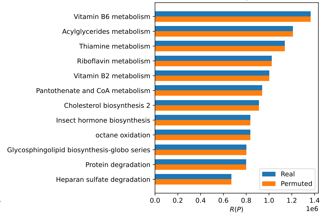
C Distribution-matched permutation control
