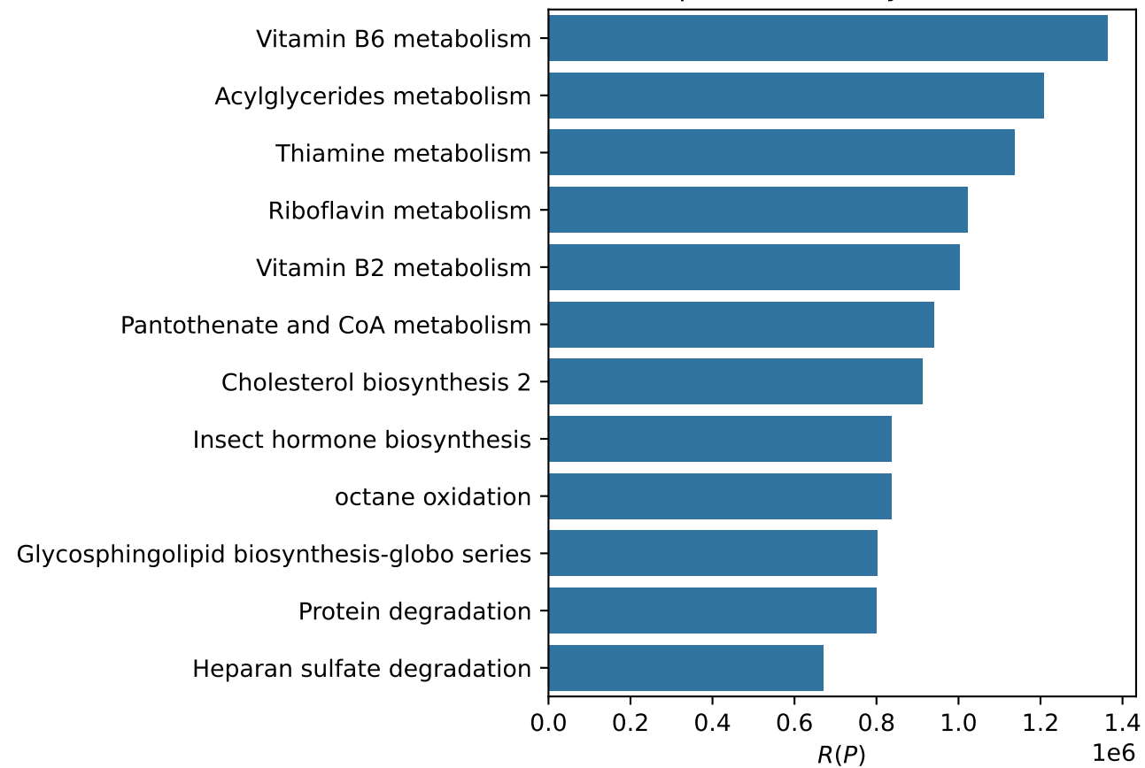
B Top rewired subsystems (real)
