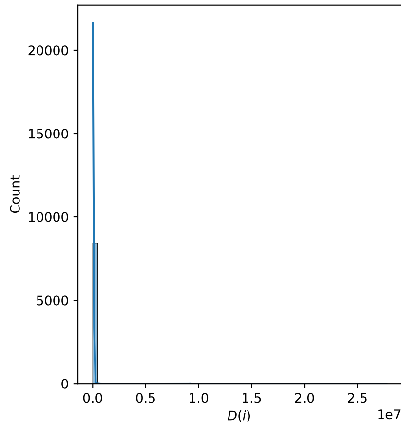
A Metabolite-level deformation D(i)
