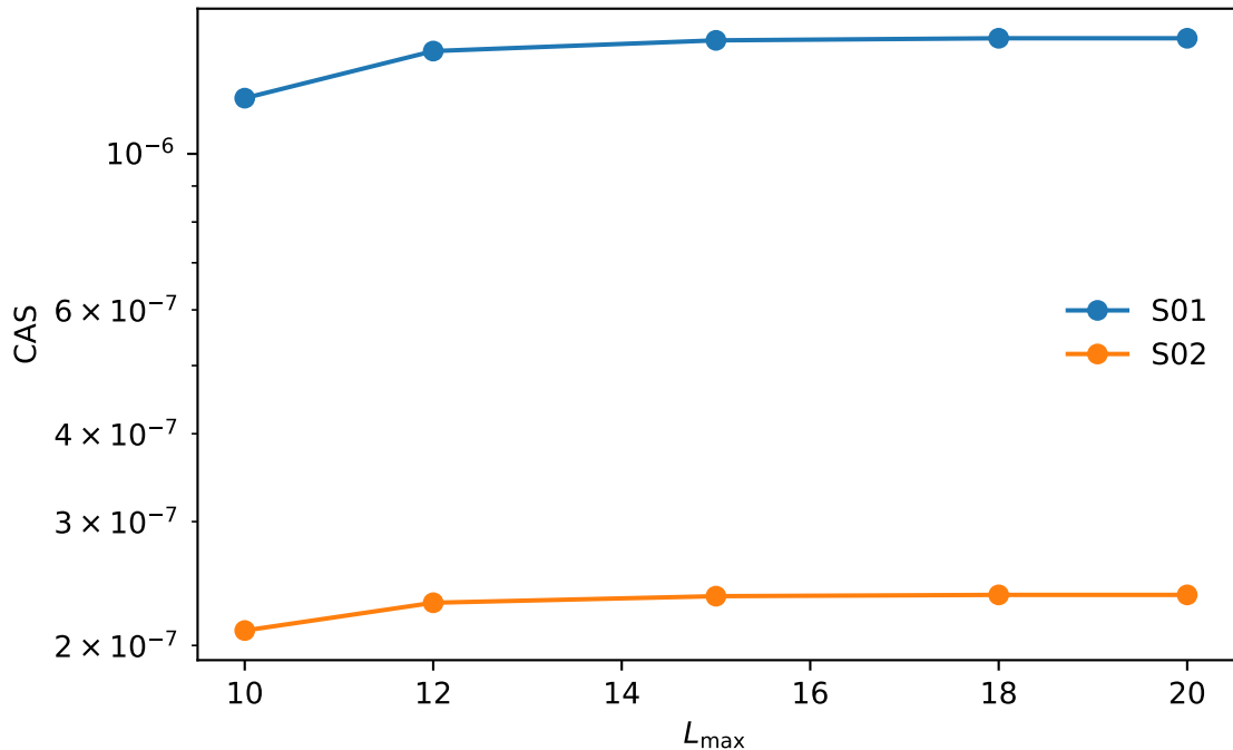
CAS stability vs insertion bound
