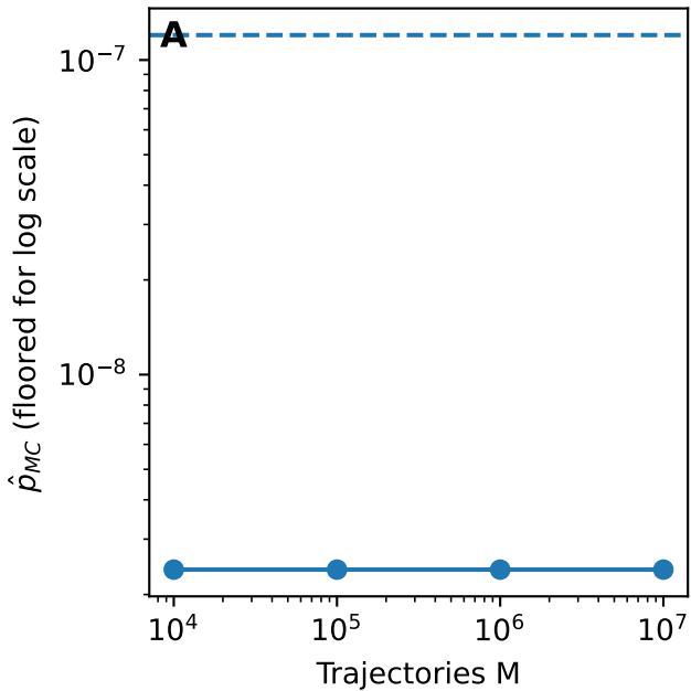
Monte Carlo vs rare-event floor
