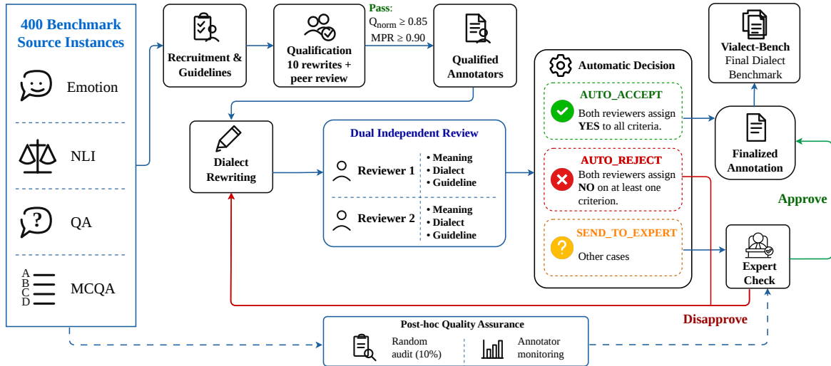
Figure 2: Overview of the annotation and quality-assurance pipeline for VialectBench .
