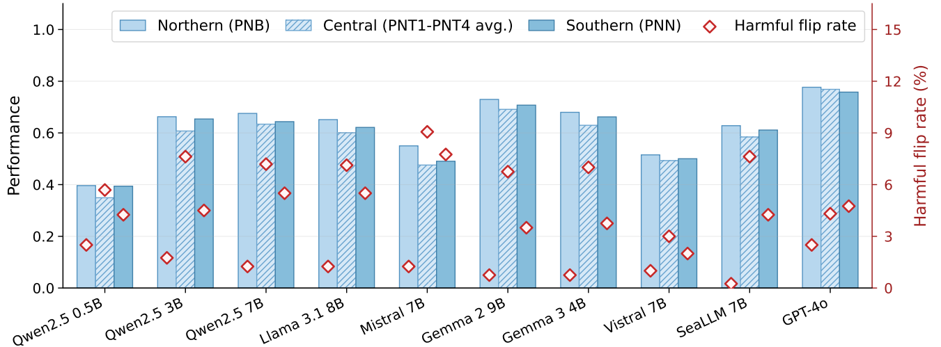
Figure 3: Regional performance (left axis) and harmful-flip rate (right axis) by model.
