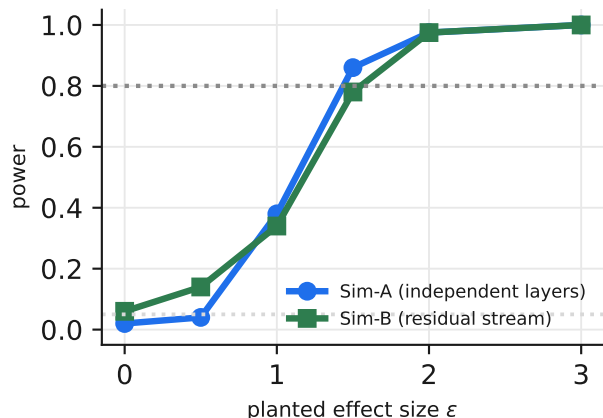
Figure 5: Power of the recentred contrast under both simulators. Both reach 0.8 near \epsilon = 1.5 and saturate by \epsilon = 3 .
