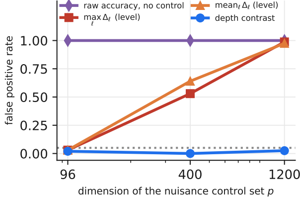
Figure 3: C1. False positive rate under a true null as the nuisance control set grows. The zero-sum contrast is flat because the control term cancels algebraically; every level-based statistic tracks the control set’s dimension.
