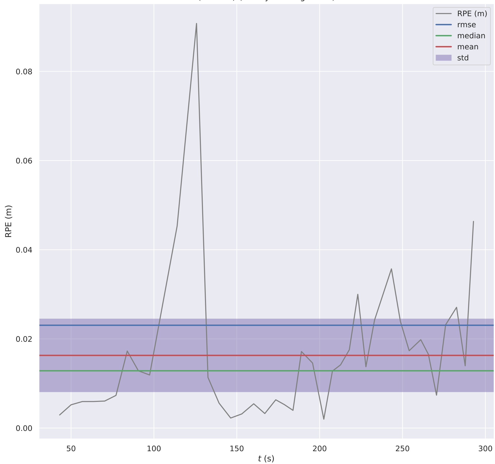
RPE w.r.t. translation part (m) for \delta = 1.0 (m) using consecutive pairs (with SE(3) Umeyama alignment)
