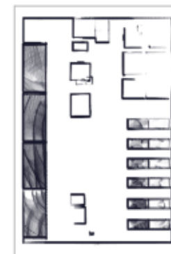
FAST-LIO
