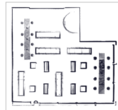
FAST-LIO
