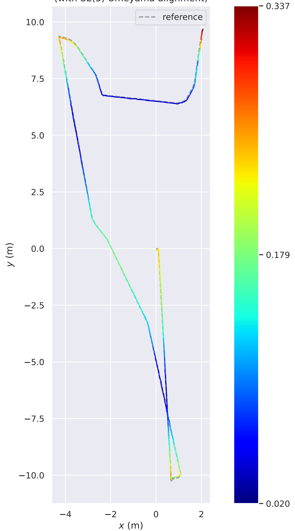
APE w.r.t. translation part (m) (with SE(3) Umeyama alignment)
