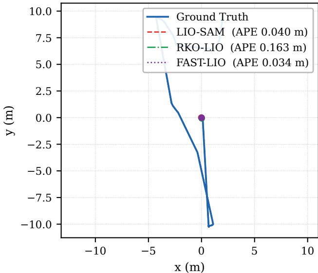
Trajectory Comparison: Warehouse 06
