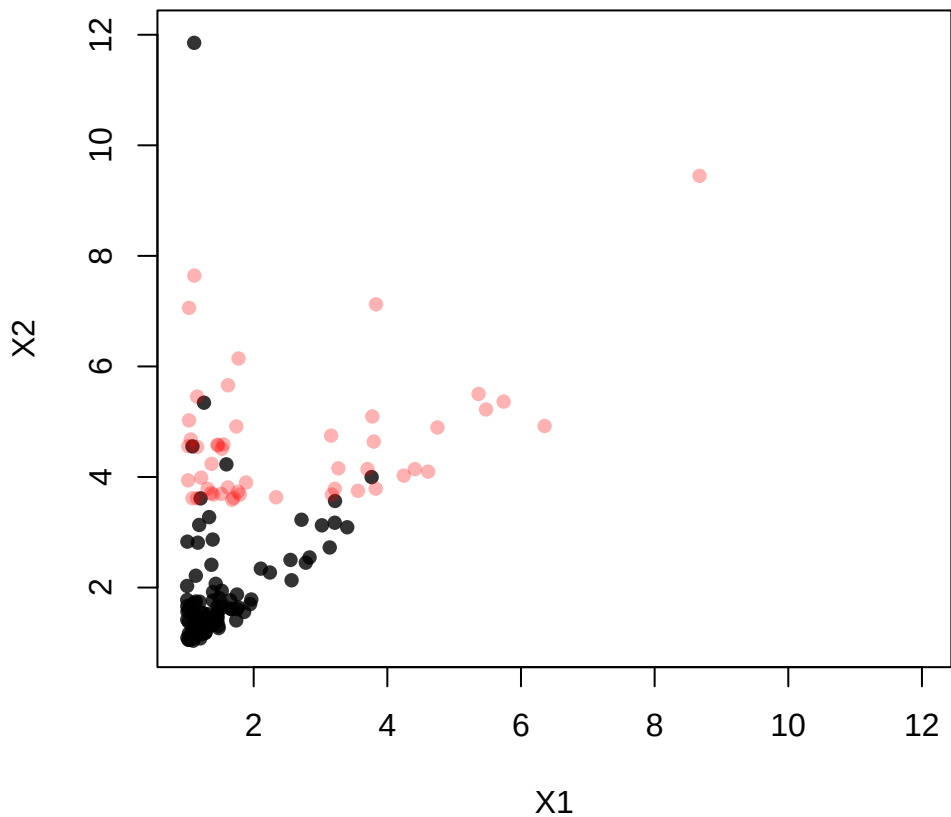
Unconditional vs Intervened ( X_2 > u )
