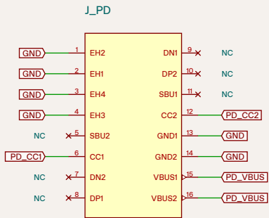
TYPE-C-31-M-12
