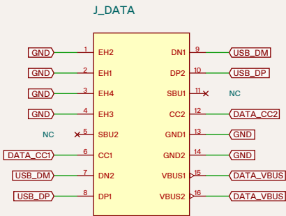
TYPE-C-31-M-12
