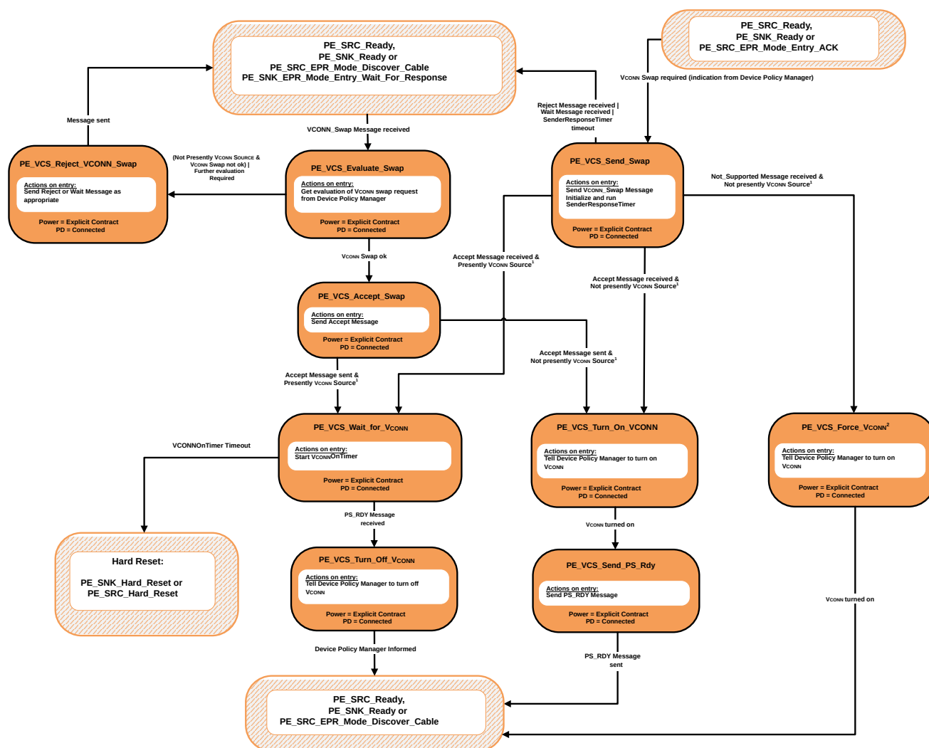
Figure 9.75. VCONN Swap State Diagram
