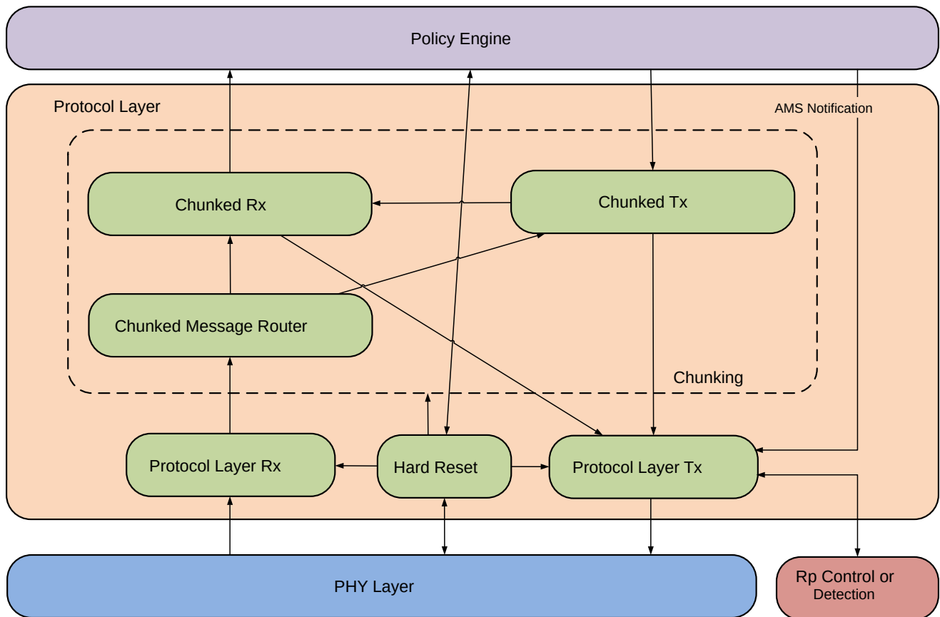
Figure 9.3. Chunking architecture Showing Message and Control Flow
