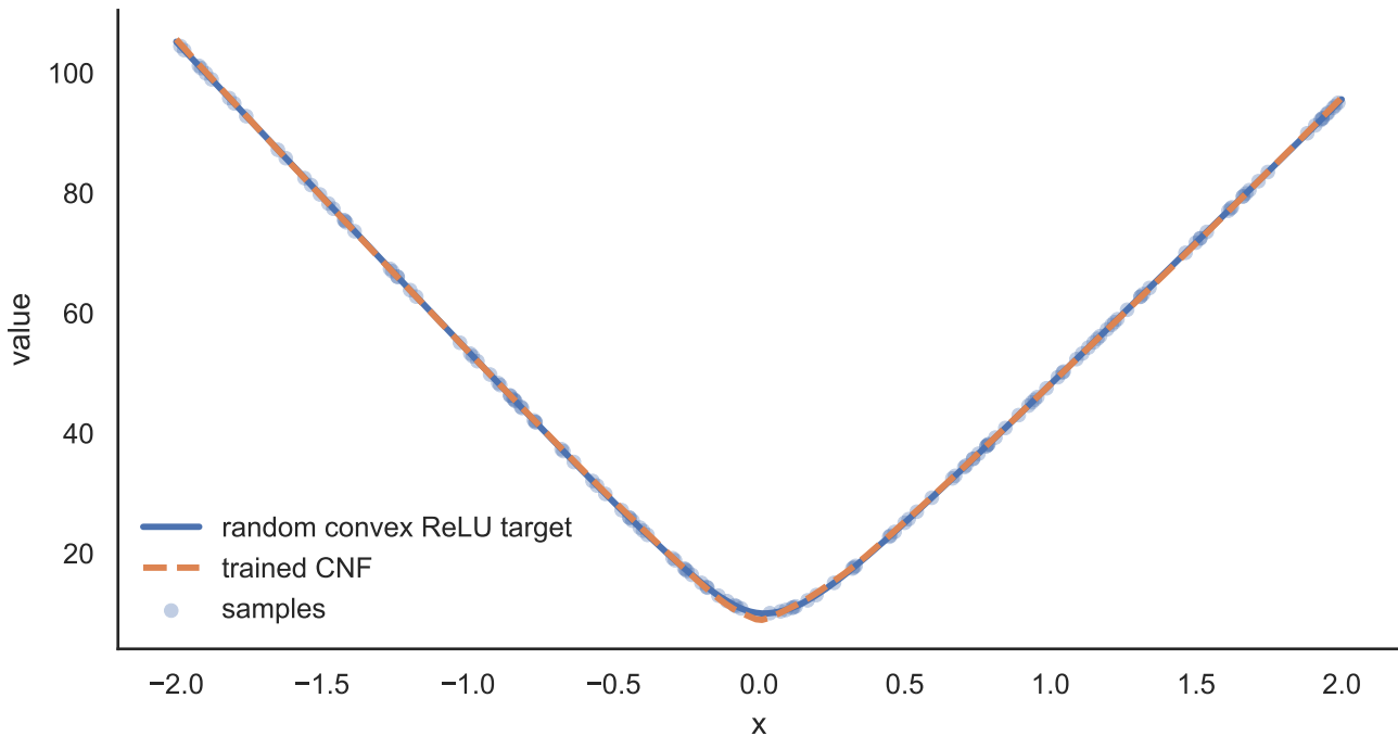
CNF fit to a random convex ReLU MLP target target params: 252,001 | CNF params: 81,402
