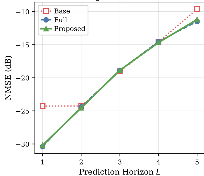
UE Speed = 12 km/h
