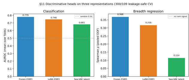
Figure 7. Added 2026-06-19. Classification AUROC (mean over folds) and breadth-regression pooled Spearman for the three representations.
