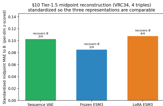
Figure 6. Added 2026-06-19. Standardized midpoint distance to the known VRC34 intermediate across the three representations (recovers- B count annotated).
