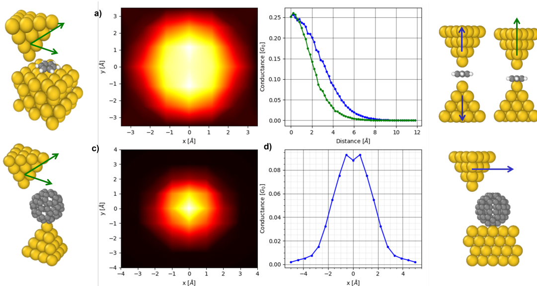
Figure 6: Examples of advanced-functionality outputs. (a) Transmission contour map from a grid scan of benzene on a gold slab. (b) Transmission as a function of electrode separation from a pull sequence on benzene, comparing the case where both electrodes move symmetrically (blue) with the case where only the top electrode moves (green). (c) Grid scan of a C 60 fullerene on a gold tip. (d) Single-line scan over a fullerene on a slab, showing the transmission profile along the scan direction.
