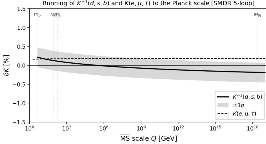
Figure 1: RG running up to Planck Mass
