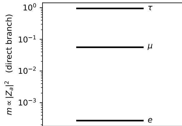
(b) leptons: direct coupling
