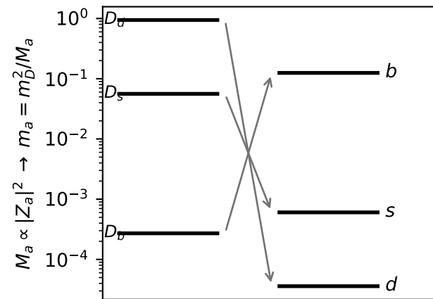
(c) down quarks: seesaw inversion
