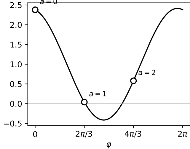
(a) self-dual amplitude, three family samples
