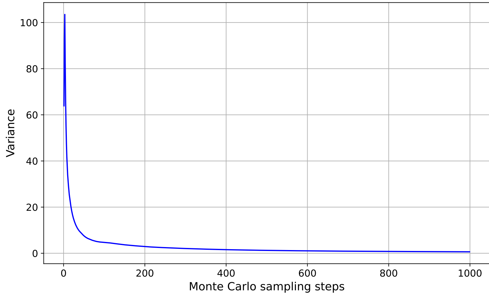
Variance of the Shapley values
