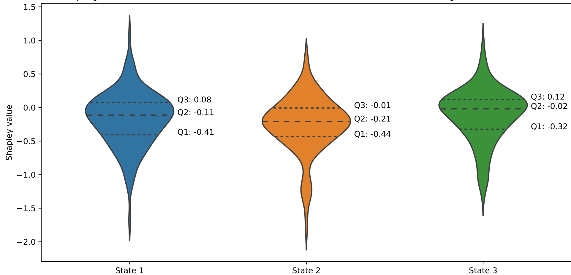
Shapley Value Distributions Across Different Initial States for Structurally Dissimilar Linkers
