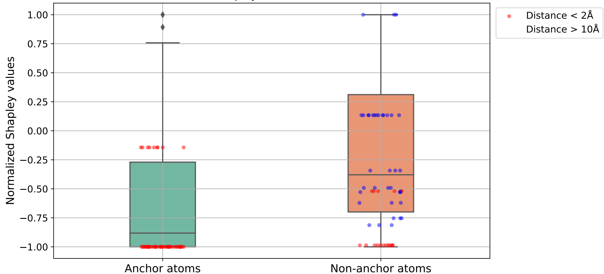
Normalized Shapley Values (Coulomb Matrix)
