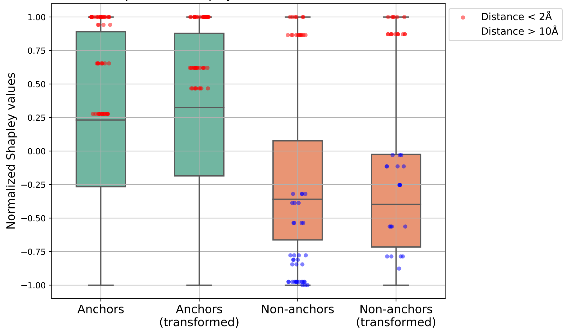
Comparison of Shapley Values (Hausdorff Distance)
