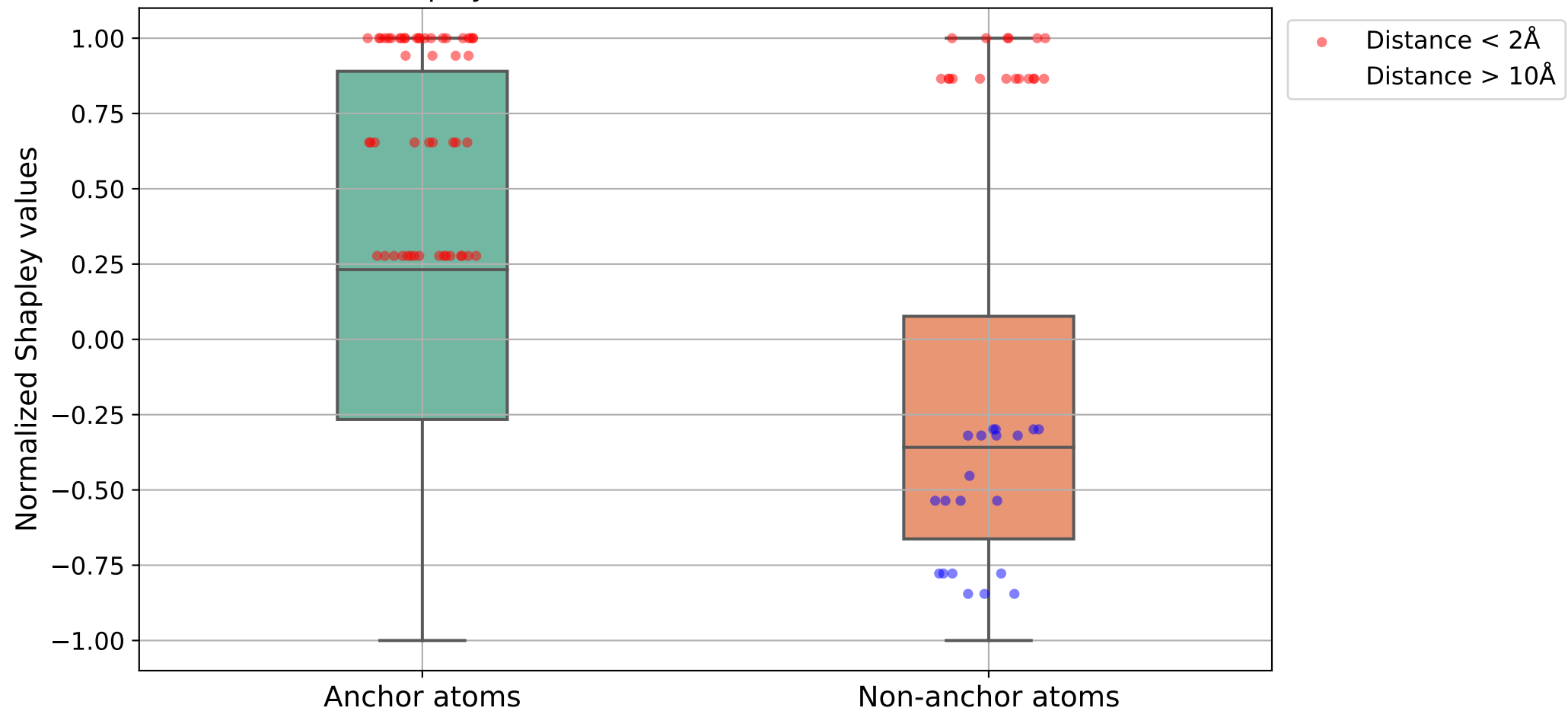
Normalized Shapley Values After Transformations (Hausdorff Distance)
