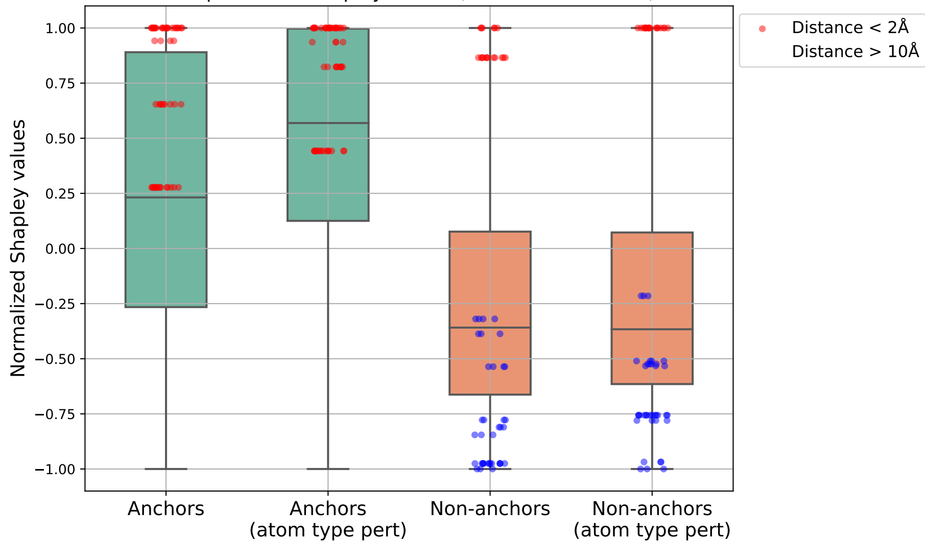
Comparison of Shapley Values (Hausdorff Distance)
