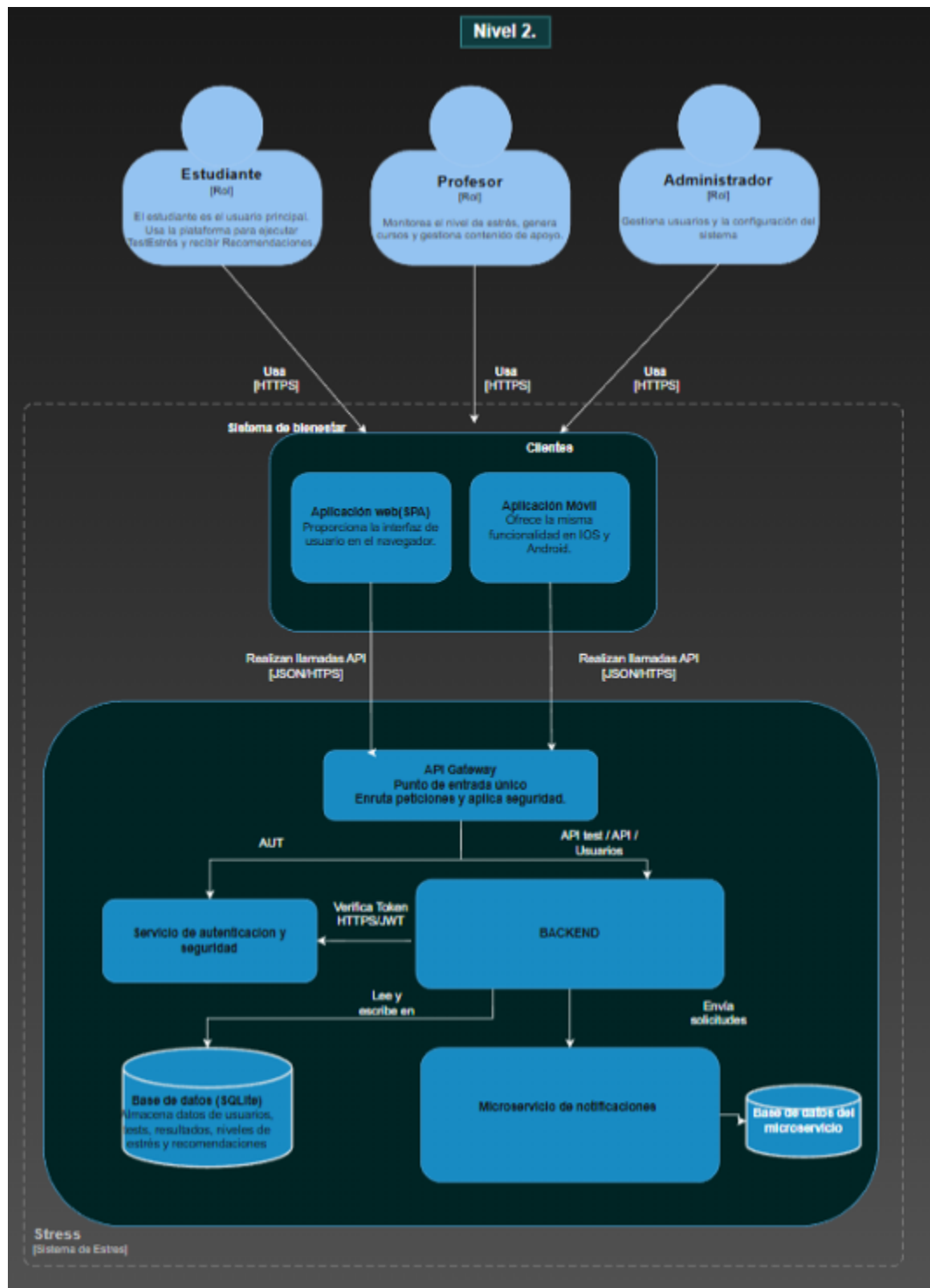
Figure 2: Diagrama de Contenedores (Nivel 2)
