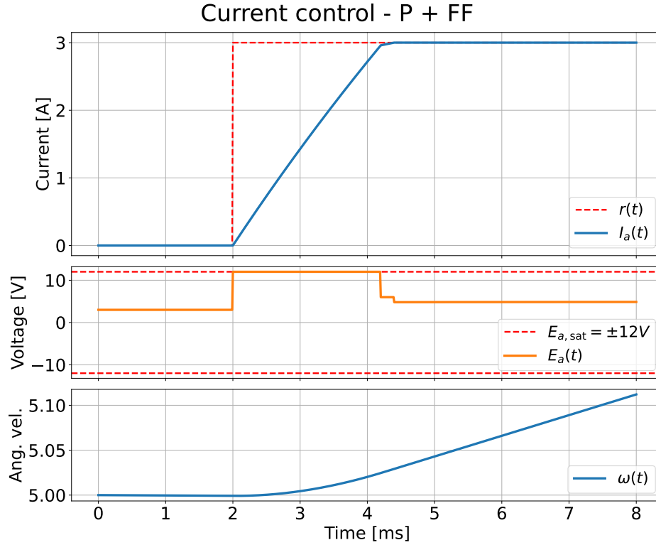
Figure 4.1: Simulation of the P+FF current controller with T_s = 0.2 ms.
