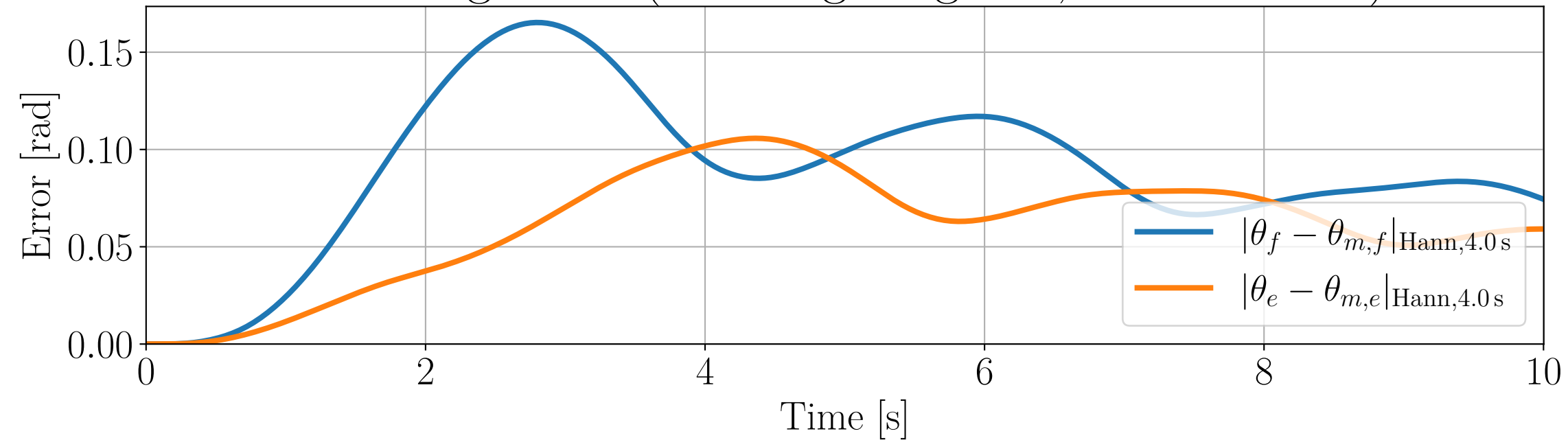
Tracking Error (Hanning-weighted, 4.0 s window)
