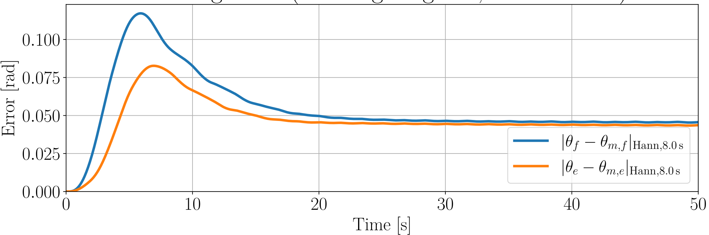
Tracking Error (Hanning-weighted, 8.0 s window)
