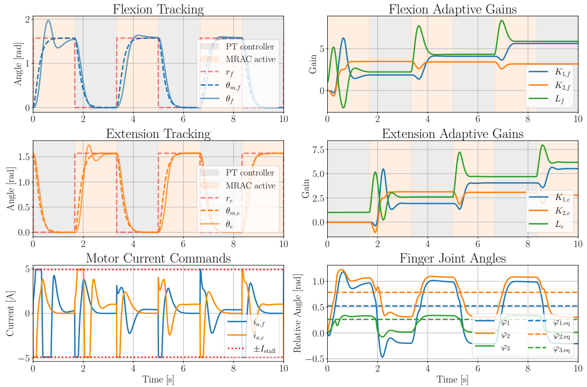
Figure 4.7: Simulation results of the MRAC scheme for flexion and extension motor over 10 s.
