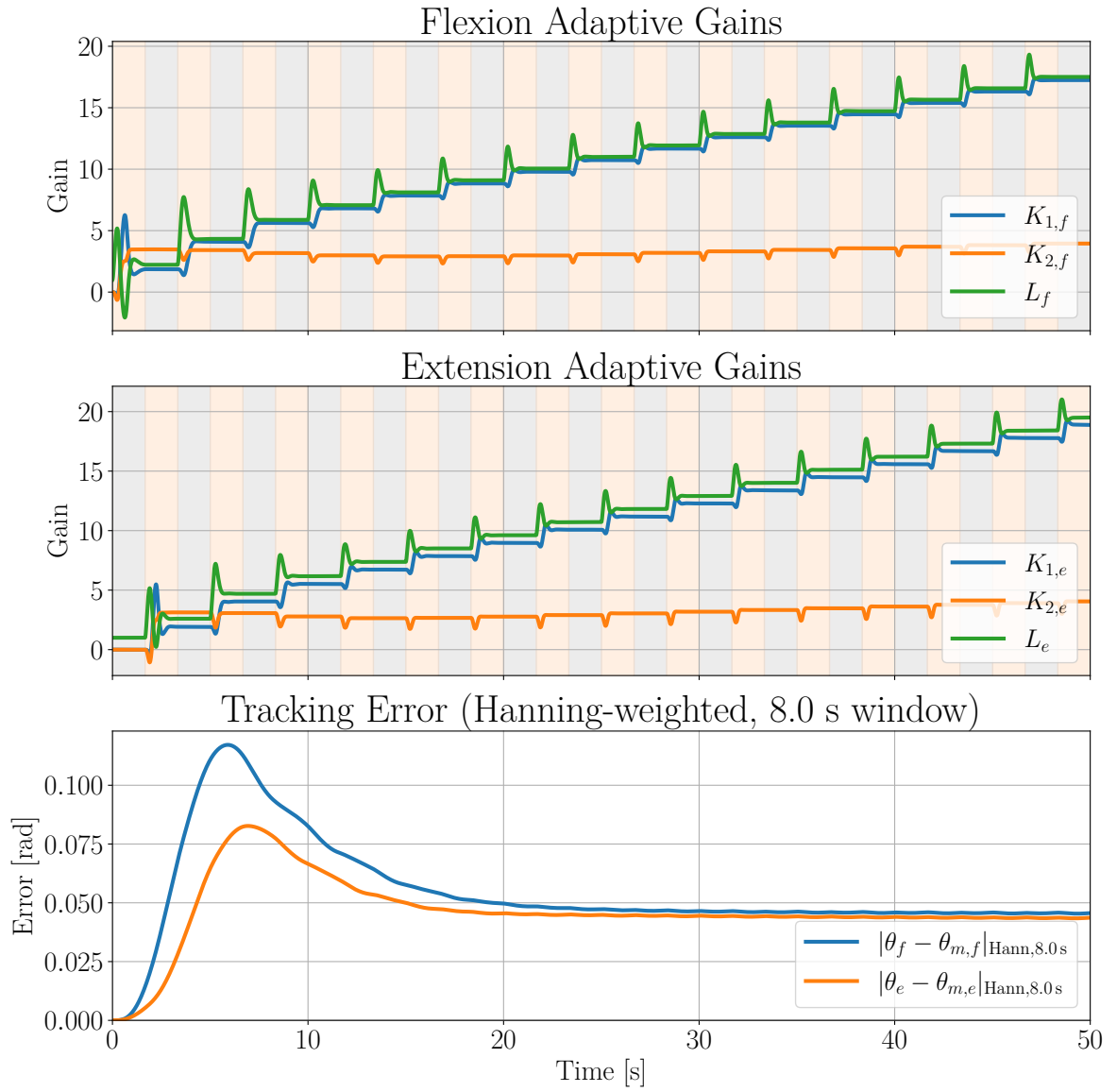
Figure 4.8: Adaptive gains and error over time for MRAC scheme for 50 s.
