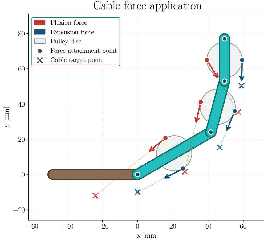
Figure 3.5: Force application on the finger. Shows how the force from the flexion and extension motors gets distributed after the whiffletrees.
