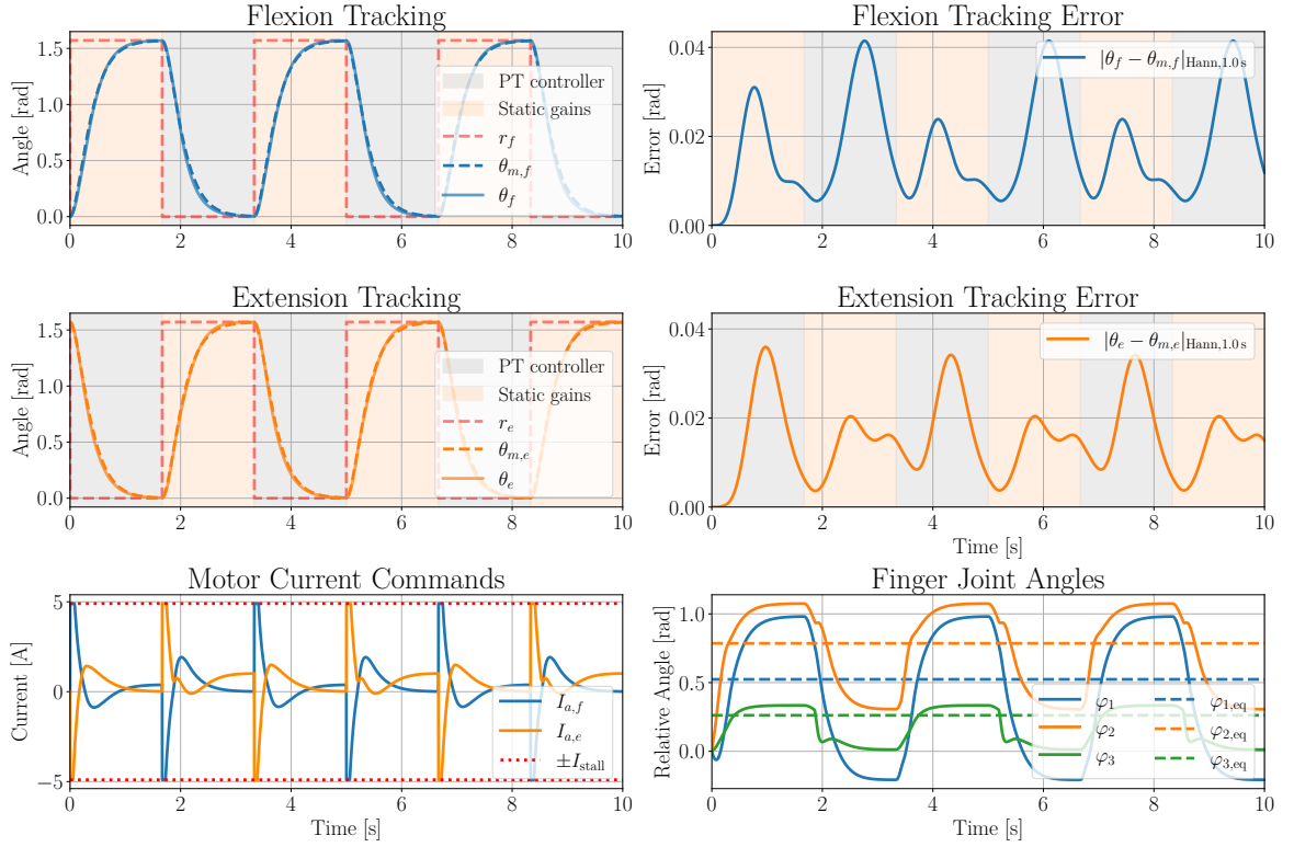
Figure 4.11: Simulation results of the MRAC scheme for flexion and extension motor over 10 s, with the adaptive gains found in Figure 4.10 after 100 s as static gains instead of adaptive.
