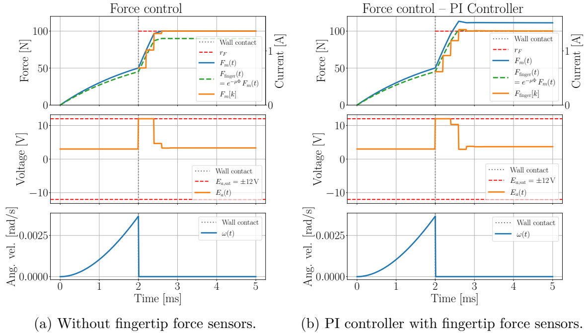
Figure 4.7: Force control with friction. With and without force sensors in fingertips. Both controllers have T_s = 0.2 \text{ ms} .
