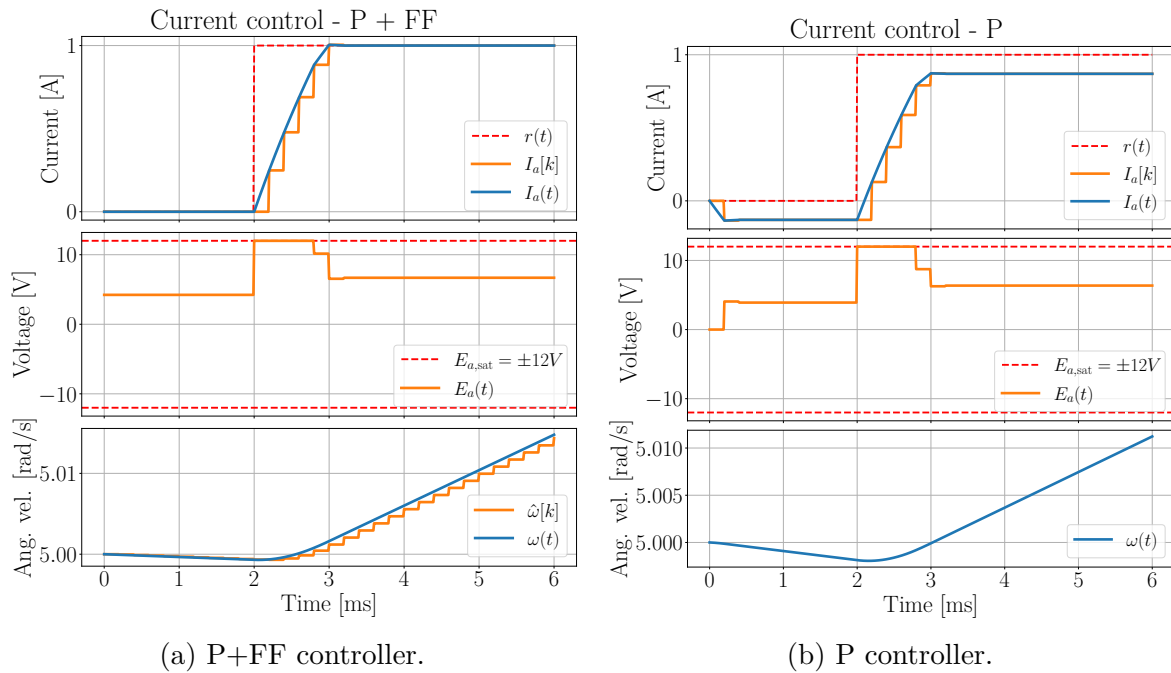
Figure 4.1: Armature current step response for discrete-time P+FF and P controllers tracking a 1 A reference, with T_s = 0.2 ms and initial motor speed \omega_0 = 5 \text{ rad s}^{-1} .
