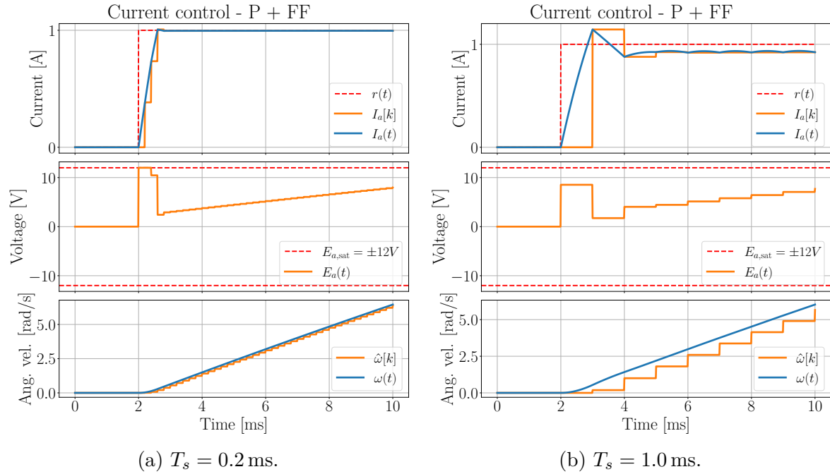
Figure 4.5: Effect of sampling time T_s on the armature current response with a smaller motor inertia J_m = 0.5 g m 2 .
