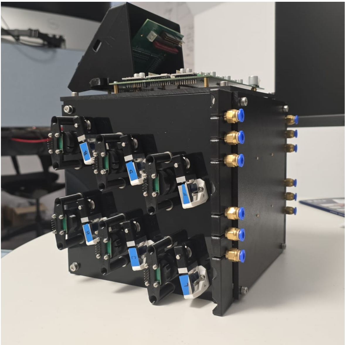
Figure 1.2: Image of the system without the cables, Bowden tubes, whiffletrees or glove. Image taken by Devon Rohlf.
