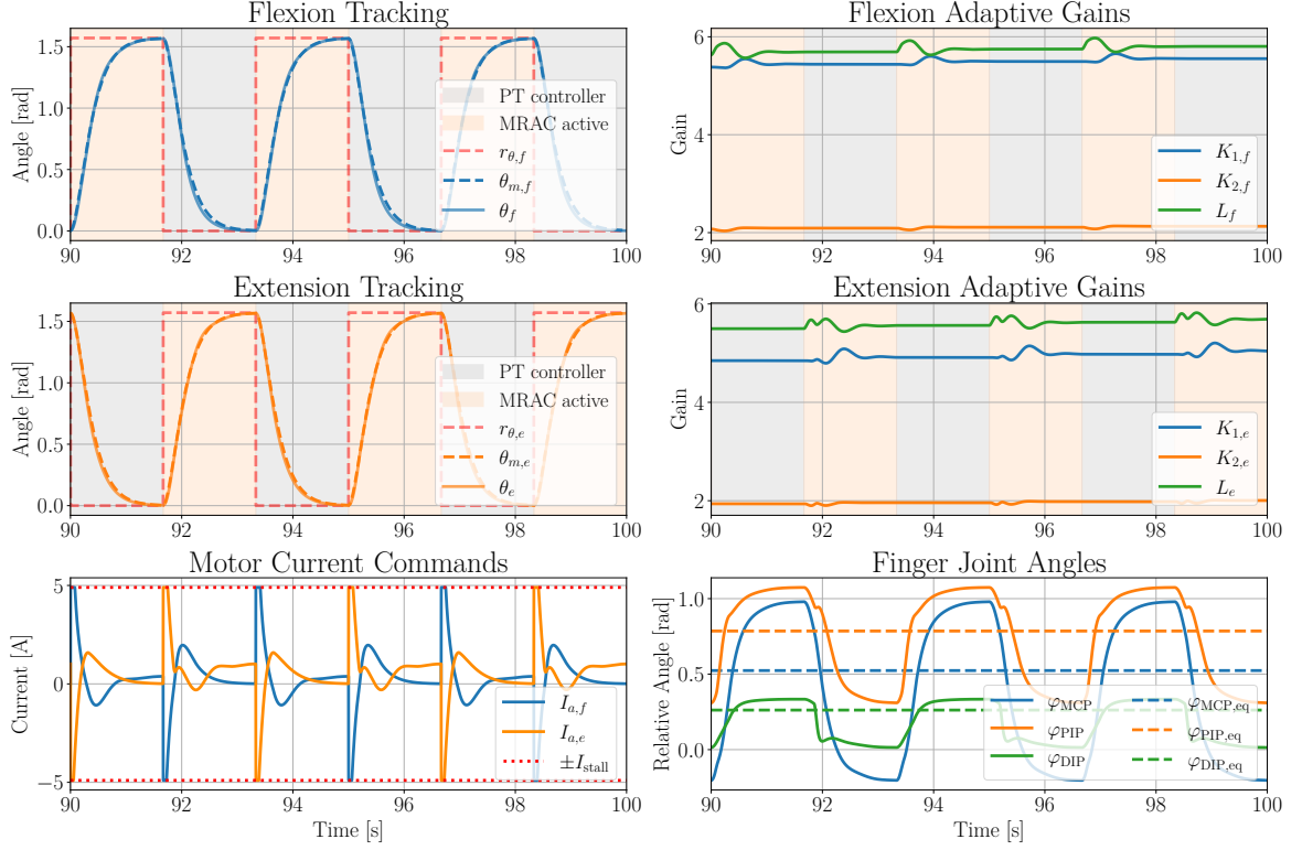
Figure 4.9: Simulation results of the MRAC scheme for flexion and extension motor after 90 s.
