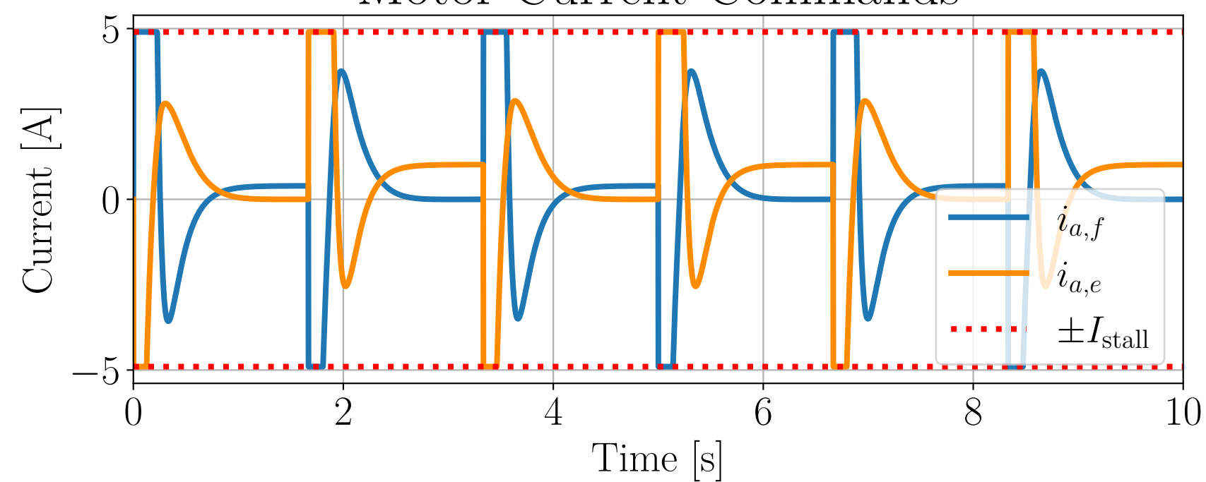
Motor Current Commands
