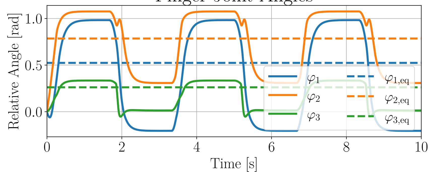
Finger Joint Angles
