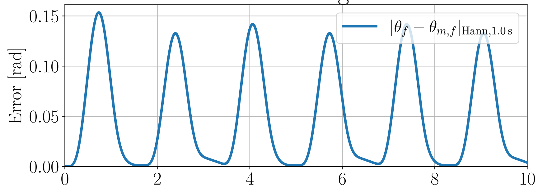
Flexion Tracking Error
