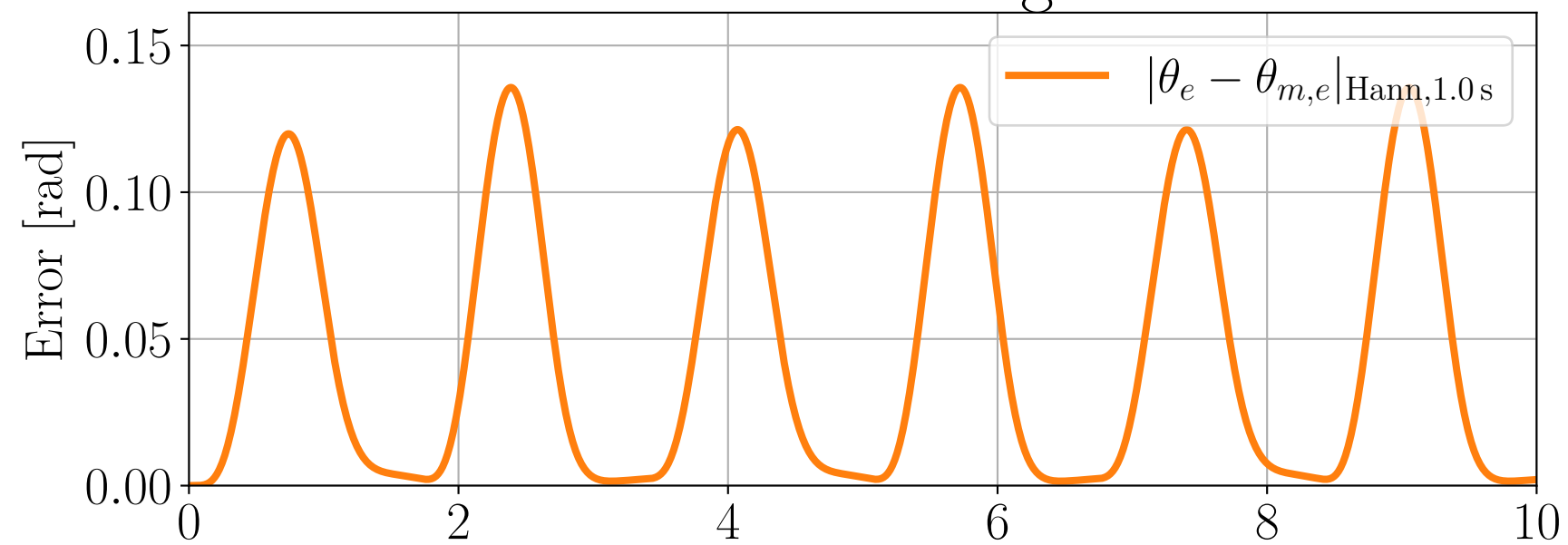
Extension Tracking Error
