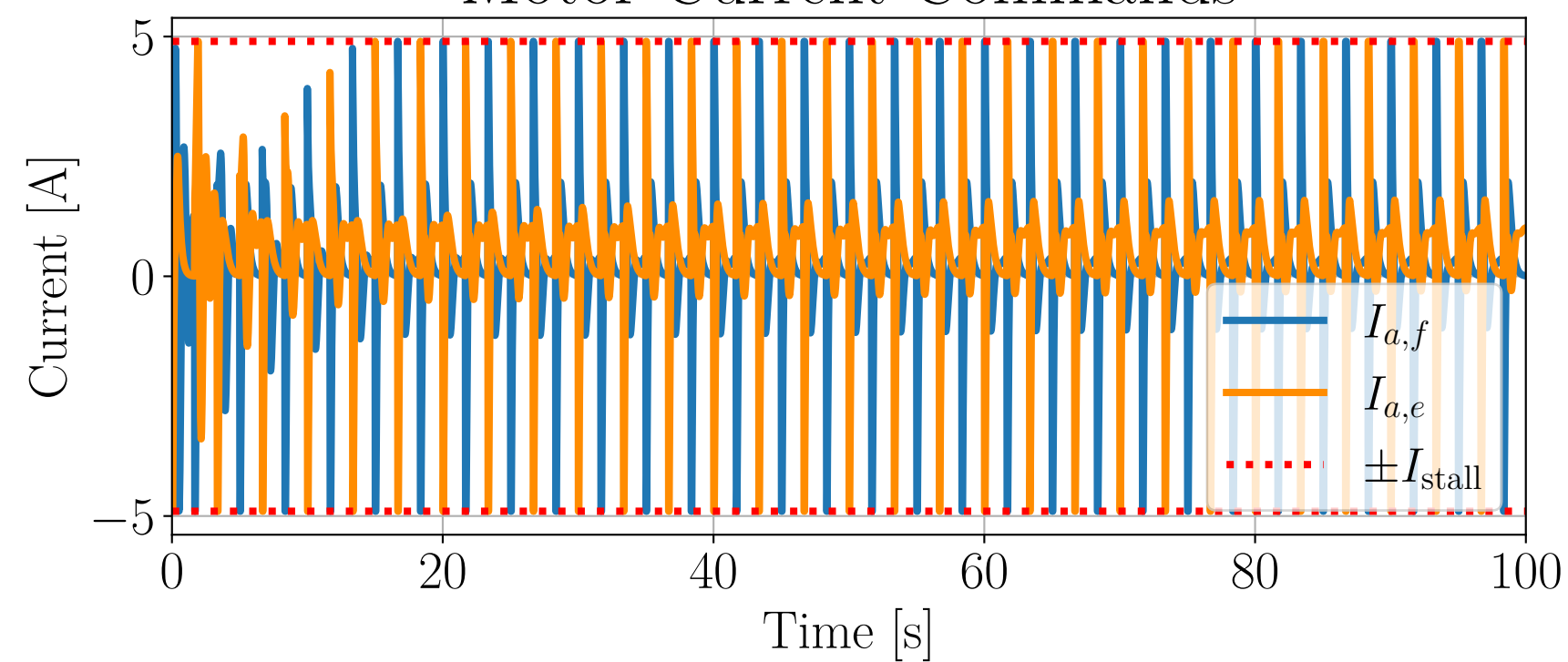
Motor Current Commands
