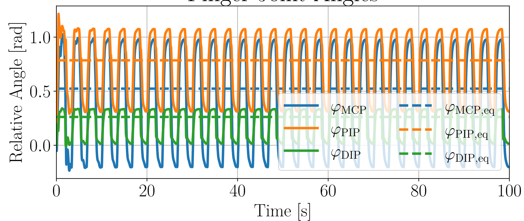
Finger Joint Angles
