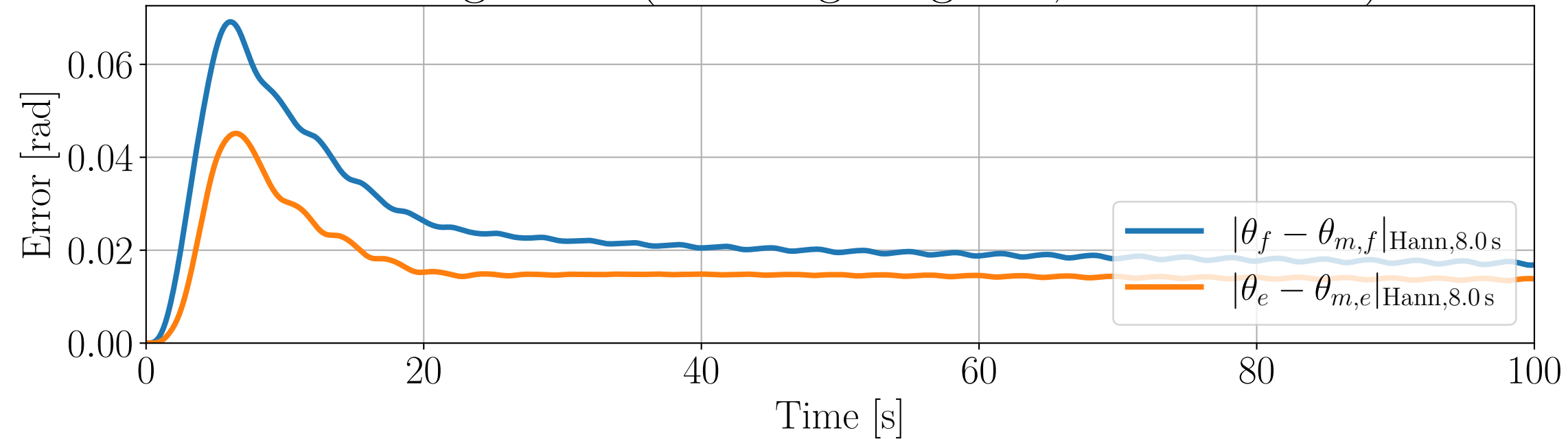
Tracking Error (Hanning-weighted, 8.0 s window)
