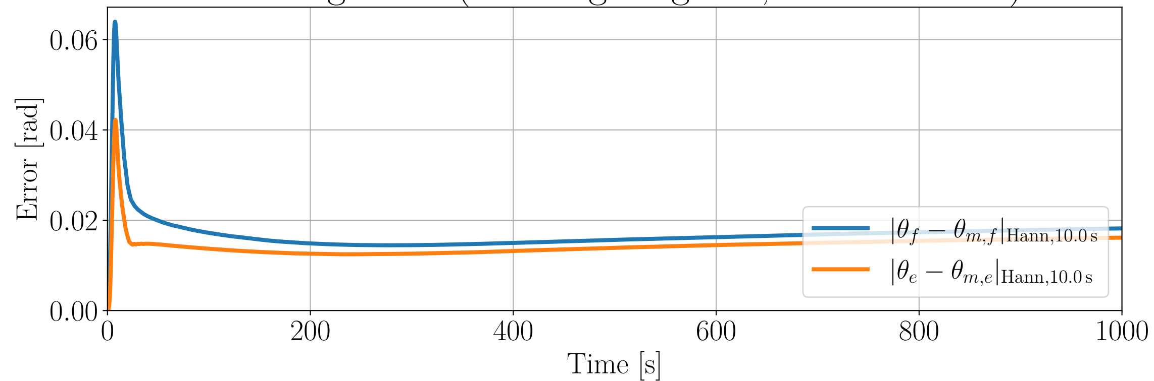
Tracking Error (Hanning-weighted, 10.0 s window)
