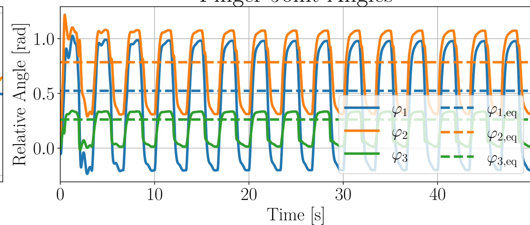
Finger Joint Angles
