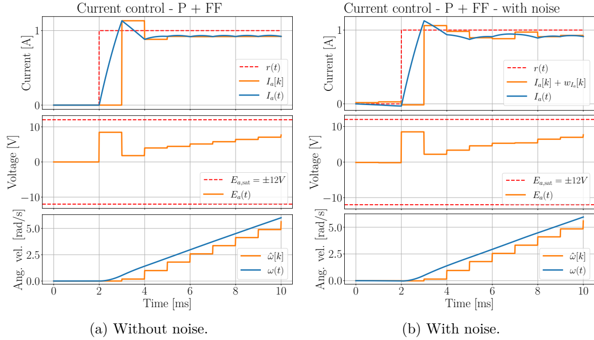
Figure 4.4: P+FF controller with and without noise, with T_s = 1.0 ms.
