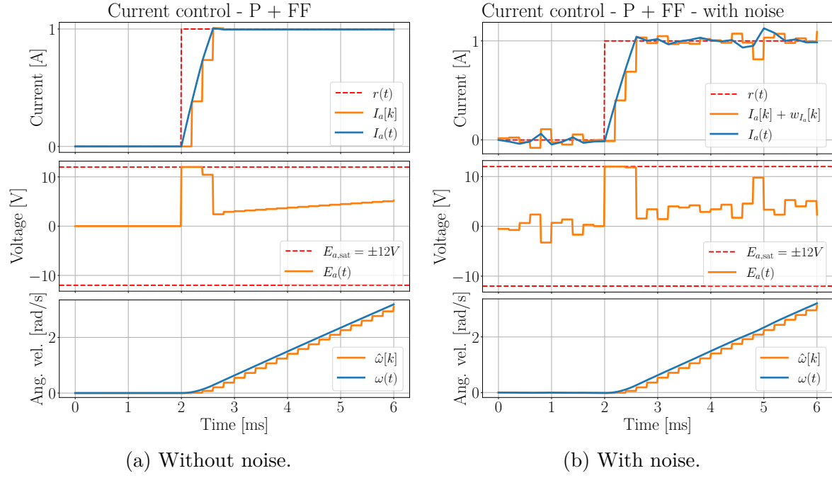
Figure 4.3: P+FF controller with and without noise, with T_s = 0.2 ms.
