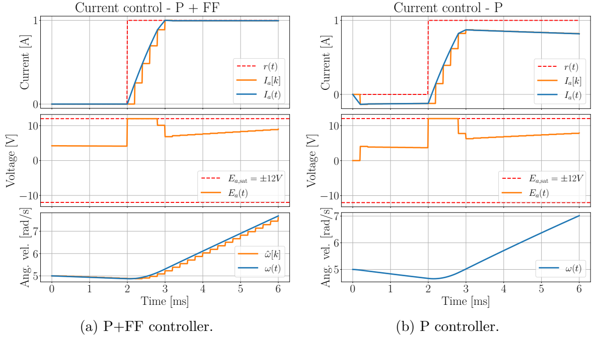
Figure 4.1: P+FF and P controllers with T_s = 0.2 \text{ ms} and \omega_0 = 5 \text{ rad/s} .
