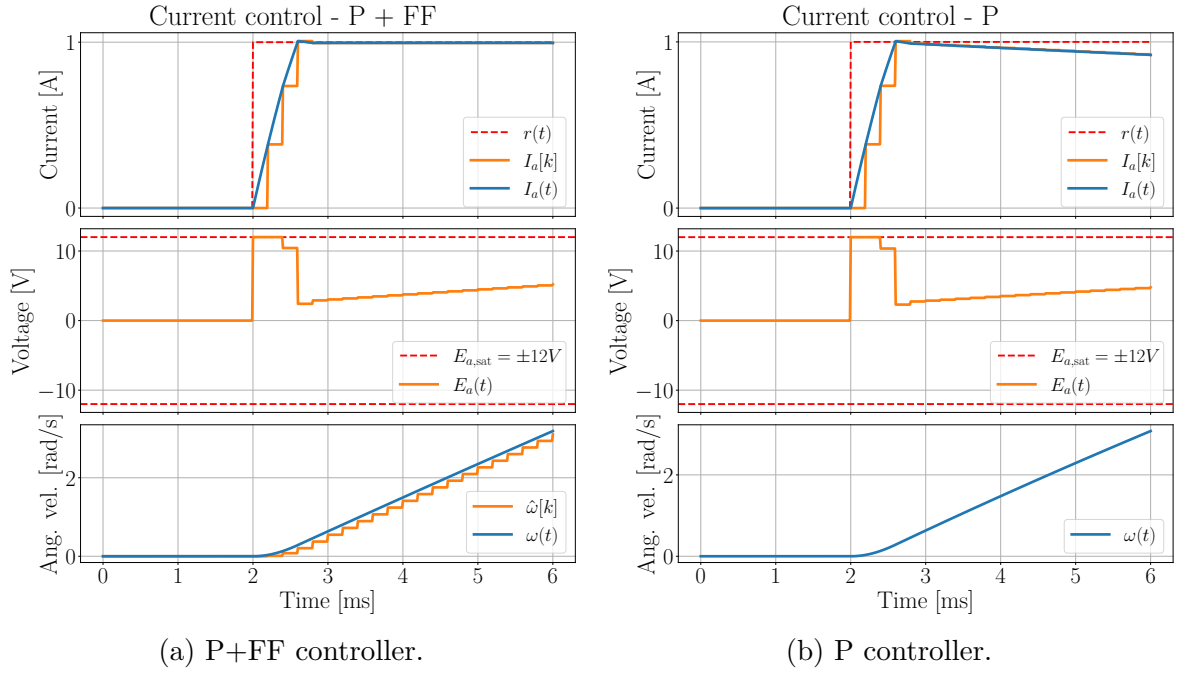
Figure 4.2: P+FF and P controllers with T_s = 0.2 \text{ ms} and \omega_0 = 0 \text{ rad/s} .
