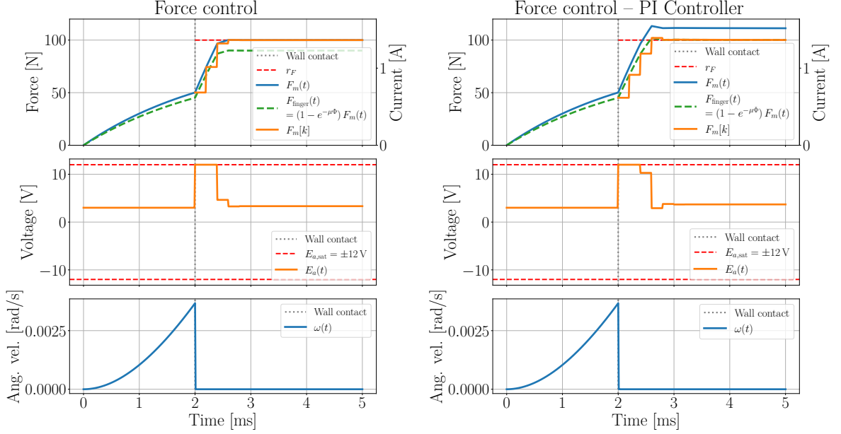
(a) Without fingertip force sensors.
