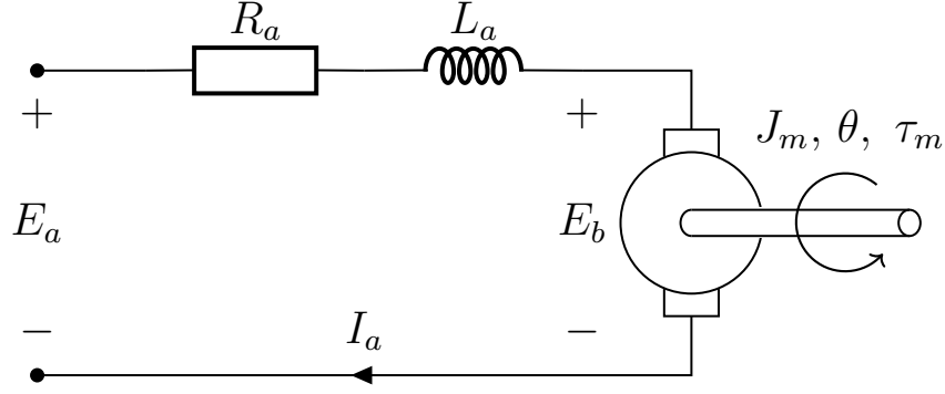
Figure 3.3: Circuit diagram of armature circuit of the DC motor model, with output torque and angular position.
