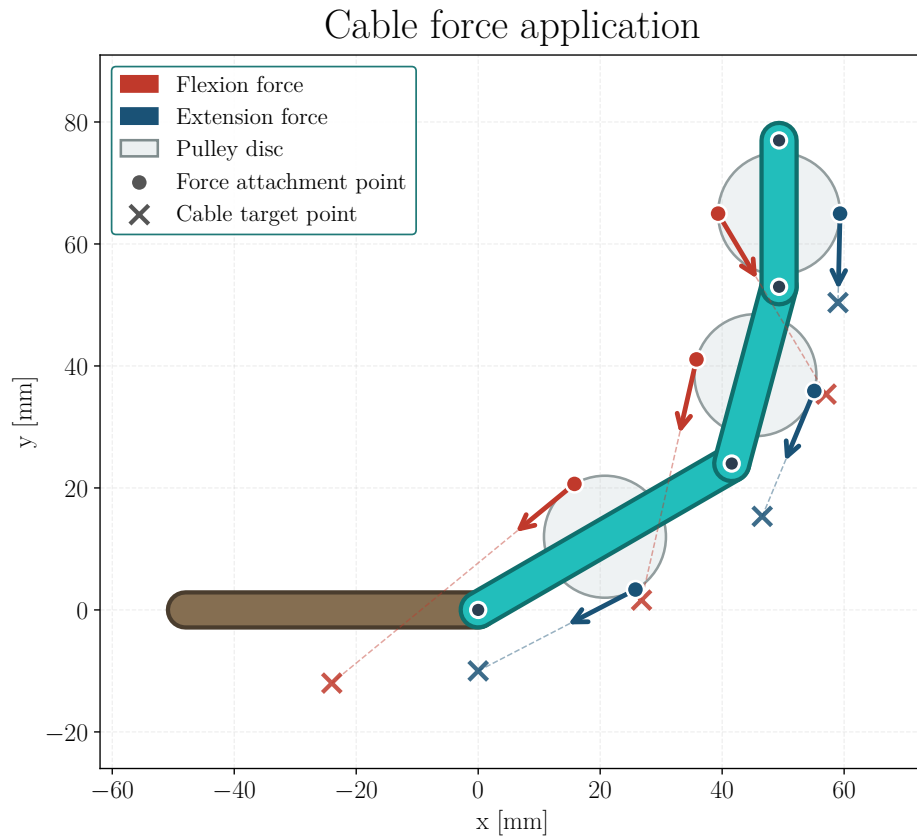
Figure 4.8: Force application on the finger. The flexion motor applies a force F_f on the flexion cable, which gets distributed to the three phalanges through the whiffle tree. Similarly, the extension motor applies a force F_e on the extension cable, which also gets distributed to the three phalanges through its own whiffle tree.
