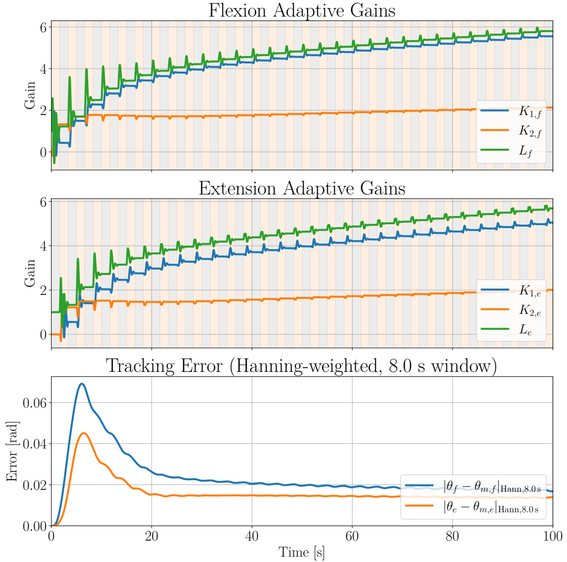
Figure 4.11: Adaptive gains and error over time for MRAC scheme for 100s, where K_1 and L keep growing together.
