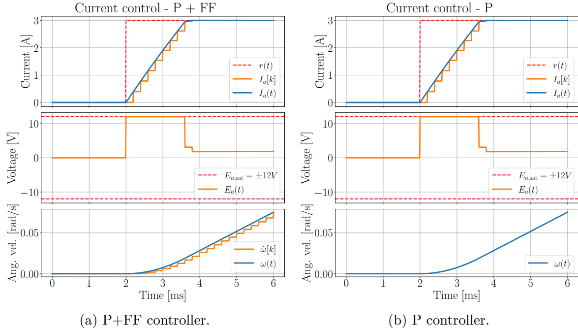
Figure 4.2: P+FF and P controllers with T_s = 0.2 \text{ ms} and \omega_0 = 0 \text{ rad s}^{-1} .
