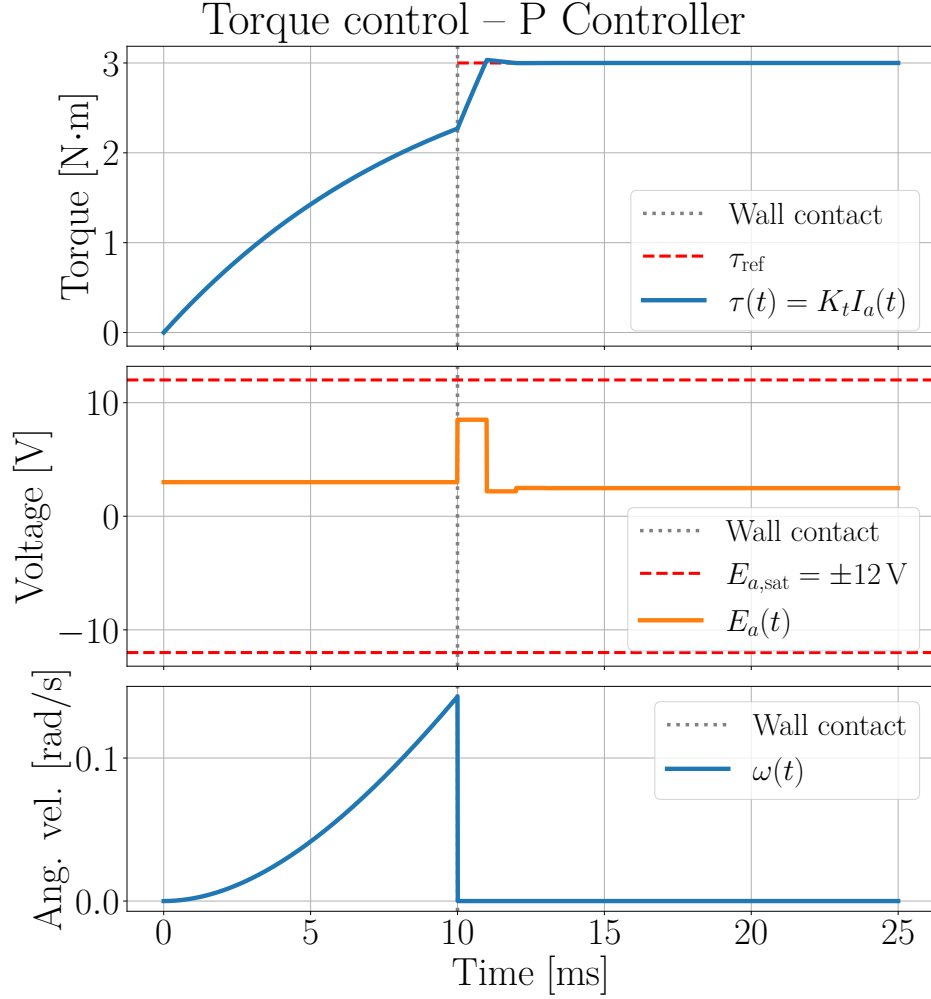
Figure 4.5: Torque control with a P controller when gripping a rigid object.
