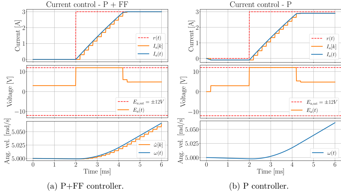
Figure 4.1: P+FF and P controllers with T_s = 0.2 \text{ ms} and \omega_0 = 5 \text{ rad s}^{-1} .
