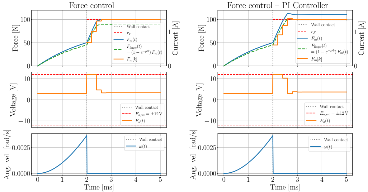
(a) Without fingertip force sensors.
