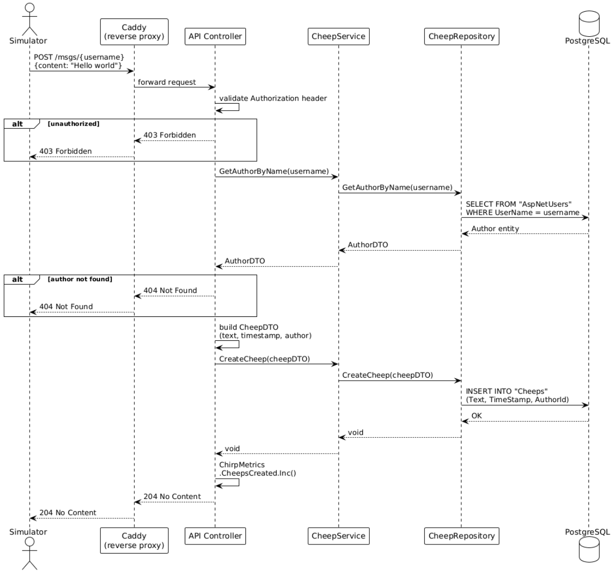
Figure 3: Component & Connector viewpoint - sequence diagram for posting a cheep.
