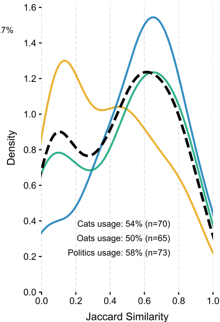
Jaccard Similarity
